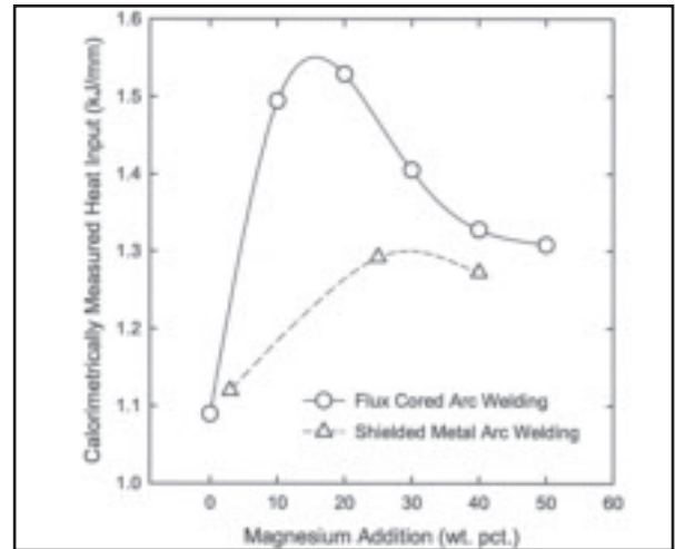
Fig. 2 — Calorimetrically measured heat input as a function of percent reactive addition for magnesium-type flux. The measured heat input of FCA and SMA welding are shown in one graph for comparison.
