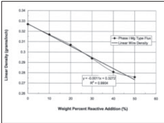
Fig. 1 — Electrode linear density as a function of wt-% magnesium-type flux addition for Part 1 study.
