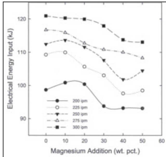
Fig. 4 — Electrical input energy as a function of weight percent addition for the magnesium-type flux at 200 to 300 in./min melting rate (85 to 127 mm/s).
