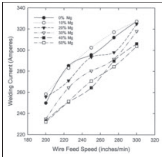
Fig. 7 — Welding current as a function of melting rate for the Part 1 magnesium-type flux-filled electrodes.
