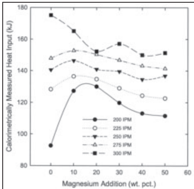
Fig. 3 — Calorimetrically measured heat input as a function of weight percent addition for magnesium-type flux at 200 to 300 in./min melting rate (85 to 127 mm/s).
