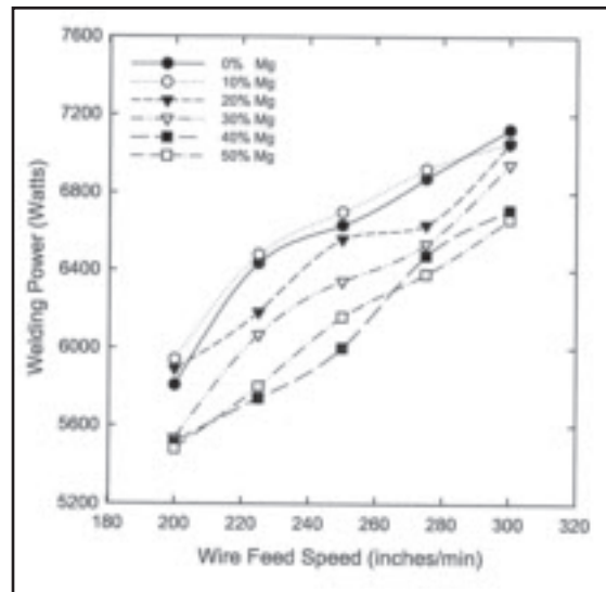
Fig. 8 — Welding power consumed as a function of melting rate for the Part 1 magnesium-type flux-filled electrodes.
