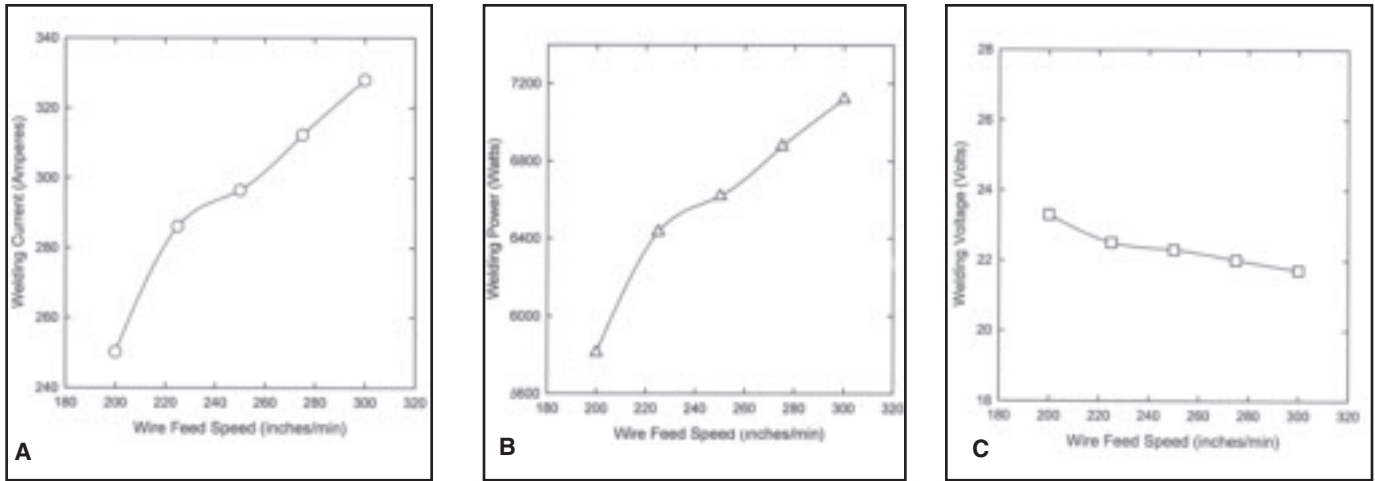
Fig. 6 — A — Welding current; B — welding power; C — welding voltage as a function of melting rate for the initial baseline composition electrode with no explicit exothermic flux addition.
