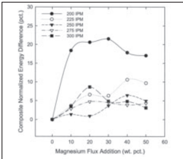
Fig. 10 — Difference in composite normalized energy value as a function of weight percent magnesium flux addition for the various melting rates.
