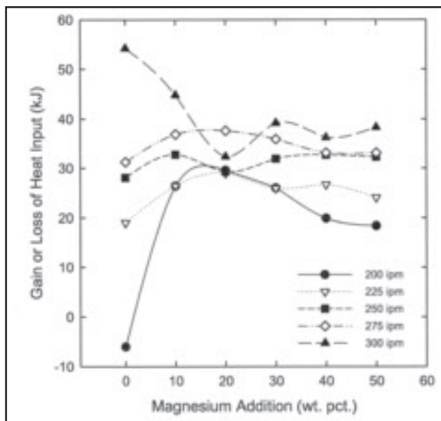
Fig. 5 — Gain or loss of heat input as a function of weight-percent addition for the magnesium-type flux at 200 to 300 in./min melting rate (85 to 127 mm/s).
