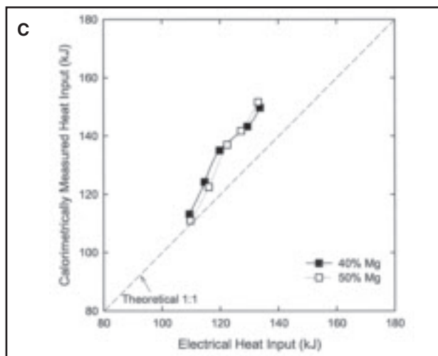
Fig. 11 — Calorimetrically measured heat input as a function of electrical heat input for: A — 0 and 10 wt-%; B — 20 and 30 wt-%; and C — 40 and 50 wt-% magnesium-type flux addition.
