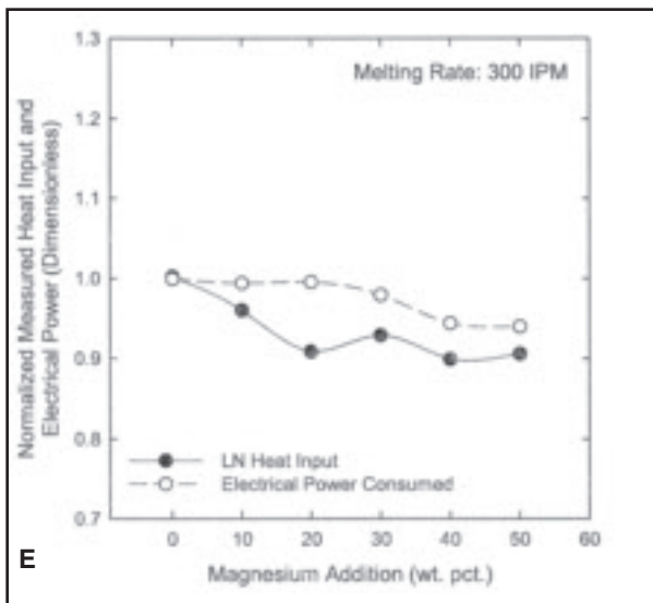
Fig. 9 — Normalized calorimetrically measured heat input and electrical power consumed for magnesium type flux at: A — 200 in./min (85 mm/s); B — 225 in./min (95 mm/s); C — 250 in./min (106 mm/s); D — 275 in./min (116 mm/s); E — 300 in./min (127 mm/s) melting rate.
