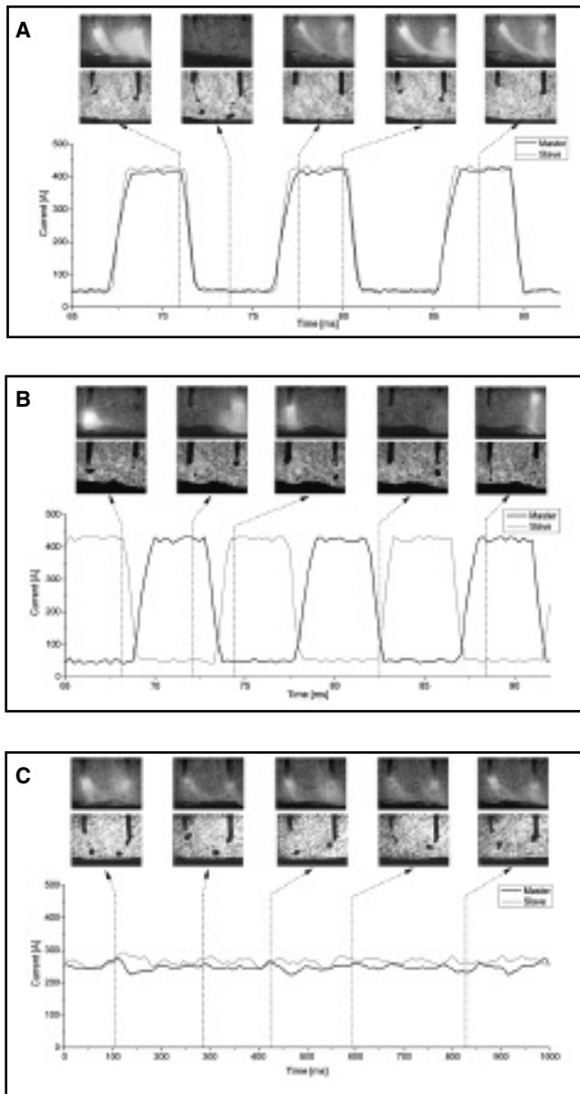
Fig. 2 — Sequential pictures of arcs and metal transfer and respective current oscillograms from Runs 1, 2, and 7. The leader wire is on the right. A — In-phase configuration, WFS_{leader} = WFS_{trailing} = 8 \text{ m/min} (Run 1); B — out-of-phase configuration, WFS_{leader} = WFS_{trailing} = 8 \text{ m/min} (Run 2); C — No pulse configuration, WFS_{leader} = WFS_{trailing} = 8 \text{ m/min} (Run 7).
