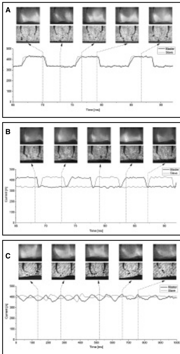
Fig. 4 — Sequential pictures of the arcs and the metal transfers and respective current oscillograms from Runs 5, 6 and 9. The leader wire is on the right. A — In-phase configuration, WFS_{leader} = WFS_{trailing} = 14 m/min (Run 5); B — Out-of-phase configuration, WFS_{leader} = WFS_{trailing} = 14 m/min (Run 6); C — No pulse configuration, WFS_{leader} = WFS_{trailing} = 14 m/min (Run 9)
