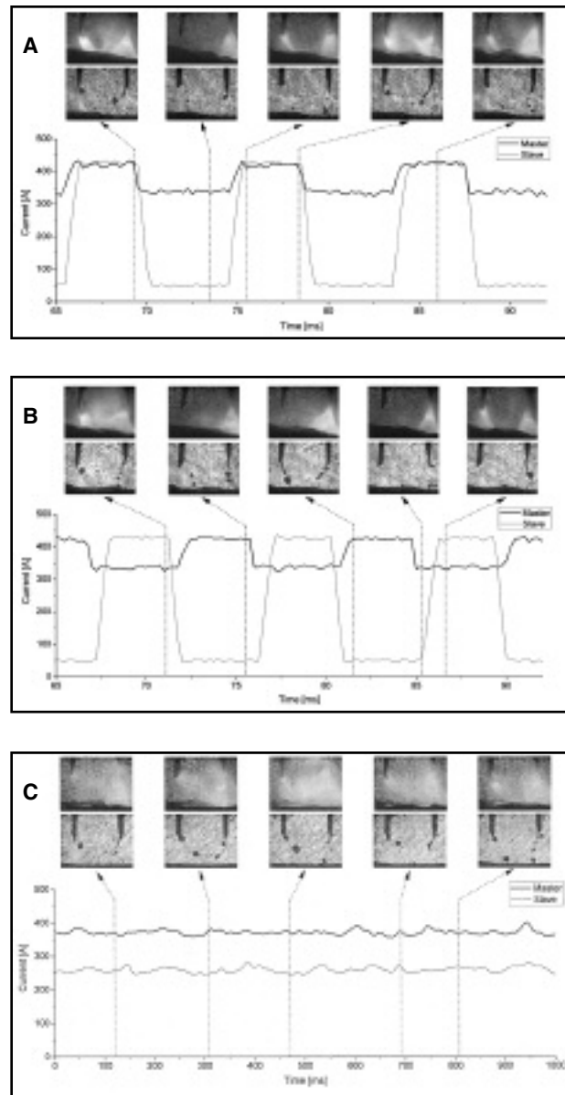
Fig. 3 — Sequential pictures of arcs and metal transfer and respective current oscillograms from Runs 3, 4, and 8. The leader wire is on the right. A — In-phase configuration, WFS_{leader} = 14 and WFS_{trailing} = 8 \text{ m/min} (Run 3); B — out-of-phase configuration, WFS_{leader} = 14 and WFS_{trailing} = 8 \text{ m/min} (Run 4); C — No pulse configuration, WFS_{leader} = 14 and WFS_{trailing} = 8 \text{ m/min} (Run 8).
