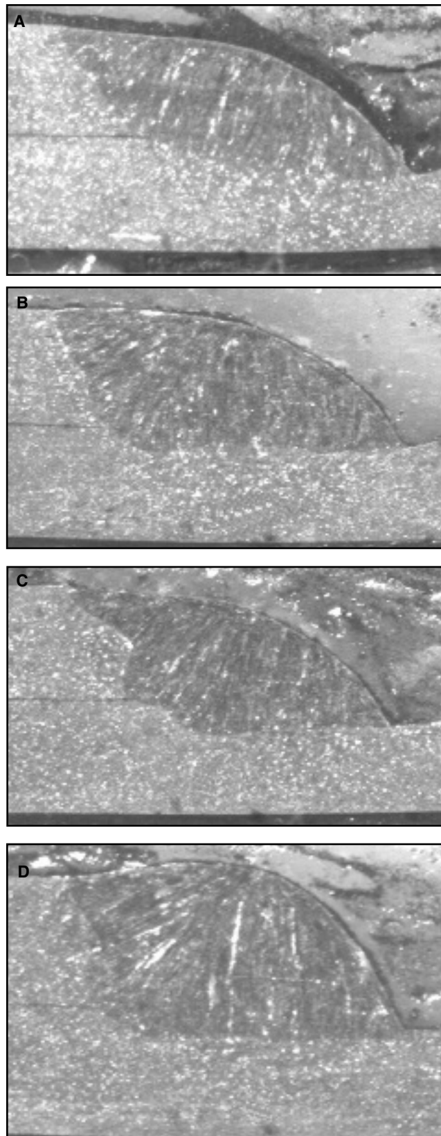
Fig. 7 — Cross sections of the beads (3-mm-thick plate overlap joints). A — Run 10, no-pulse configuration, WFS_{leader} = WFS_{trailing} = 8 m/min; B — run 11, no-pulse configuration, WFS_{leader} = 14 /min and WFS_{trailing} = 8 m/min; C — run 12, out-of-phase configuration, WFS_{leader} = WFS_{trailing} = 8 m/min; D — run 13, out-of-phase configuration, WFS_{leader} = 14 /min and WFS_{trailing} = 8 m/min.
