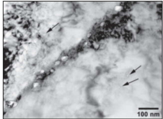
Fig. 6 — TEM image of large helium bubbles on a grain boundary and within the austenite matrix (e.g., at arrows) at about 0.010 in. (0.25 mm) below the GMA overlay interface on the 316LN plate.
