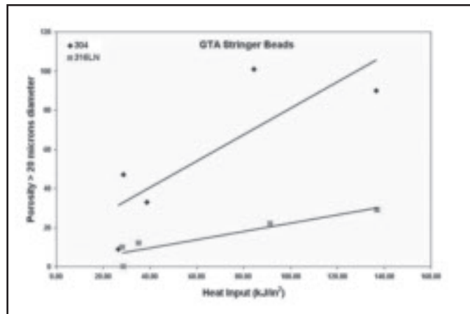
Fig. 14 — Porosity in stringer beads vs. weld heat input. More porosity in the 304 welds may indicate a higher helium content than in the 316LN plate.
