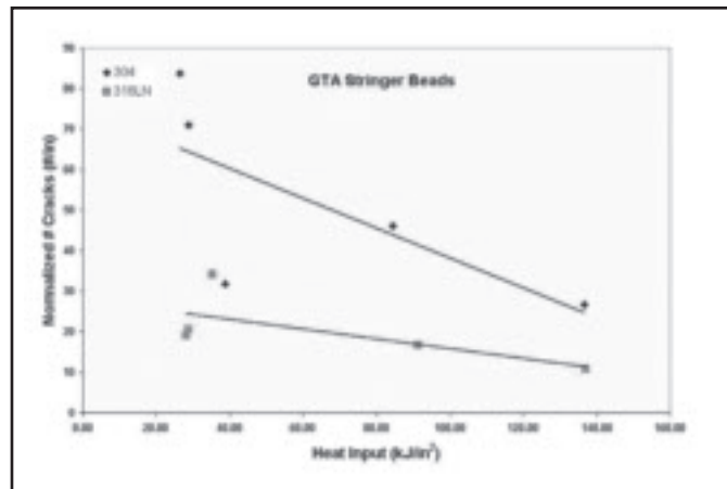
Fig. 12 — Total number of cracks per unit length of weld interface vs. heat input for the stringer beads on both plates.
