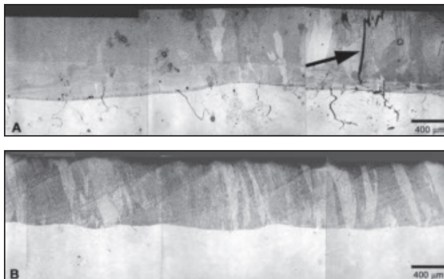
Fig. 8 — GMA overlay welds on helium-bearing plates: A — 304; B — 316LN. Much more cracking is observed in the 304 base metal. Some cracking in the weld metal can be seen at the arrow in Fig. 8A (Heat input: A — 23.4 kJ/in. 2 , B — 21.5 kJ/in. 2 ).
