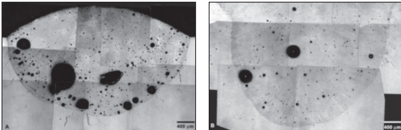
Fig. 10 — Cross-sections of stringer beads: A — 304; B — 316LN. These images further exemplify the differences in the GTA welds observed in the two steels. (Heat input: A — 84.5 kJ/in. 2 , B — 91.3 kJ/in. 2 ).
