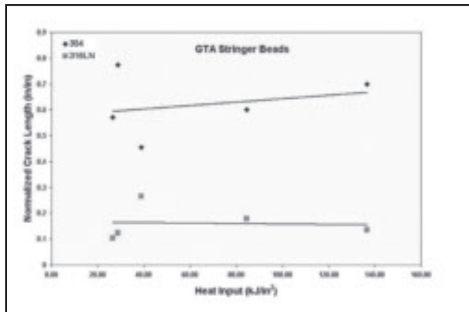
Fig. 13 — Normalized crack length vs. weld heat input for the stringer beads on both steels.
