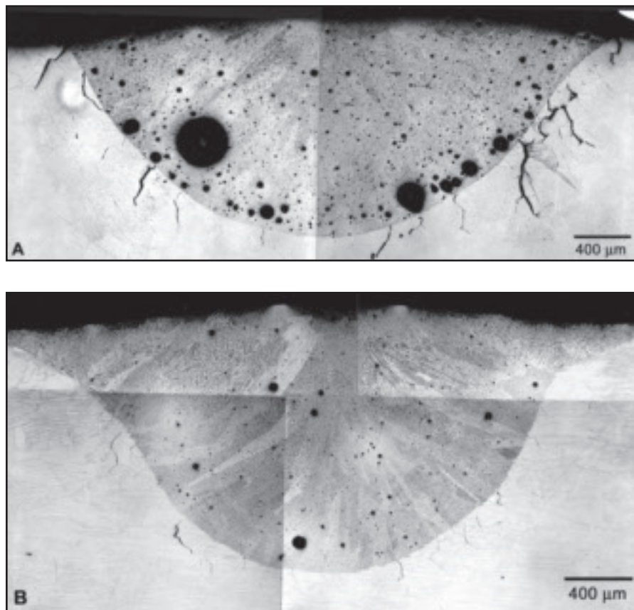
Fig. 9 — Cross sections of stringer beads: A — 304; B — 316LN. Note the differences in the number of underbead cracks, amount (and location) of porosity, and weld pool shape between the two welds. (Heat input: A — 28.7 kJ/in. 2 , B — 28.2 kJ/in. 2 ).
