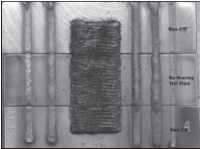
Fig. 3 — Typical weld/plate configuration. GMA overlay weld (center) with GTA stringer beads. The lower plate is the run-on tab (start of welds), the middle plate contains tritium/helium, and the upper plate is the run-off tab (end of welds).
