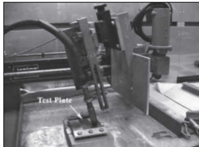
Fig. 2 — GMAW gun with oscillator. The test plate is located between the run-on and run-off tabs.
