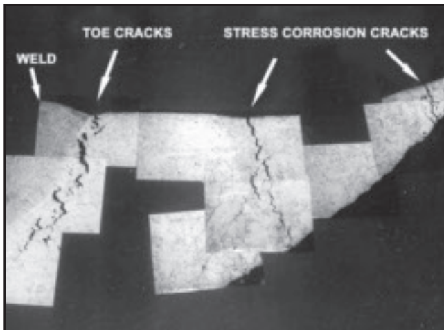
Fig. 1 — Sample removed from a reactor tank wall at the SRS showing toe cracks and stress corrosion cracks near a gas tungsten arc weld.
