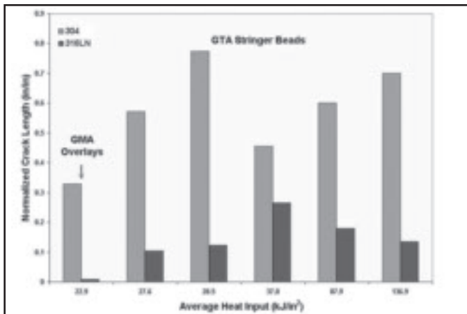
Fig. 11 — Comparison of the normalized crack length (in./in. of weld interface) for the GMA overlay welds and GTA stringer beads. Heat input values are the average of the actual heat inputs for 304 and 316LN welds at each targeted heat input level.
