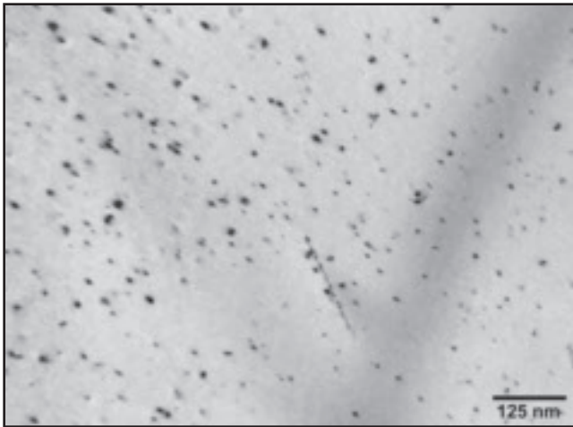
Fig. 5 — TEM image from a grain interior of the 304 material. The black dots are dislocation loops punched out by the formation of helium bubbles. Dislocation loops (or bubbles) were not observed in the 316LN.
