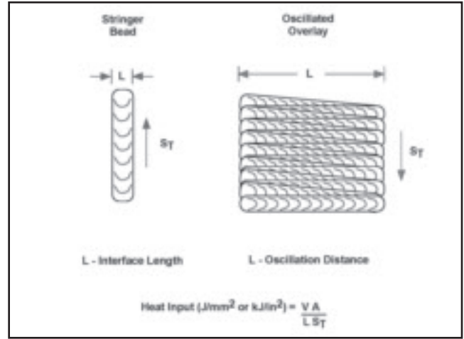
Fig. 4 — Schematic diagram illustrating the parameters used for heat input calculations for both GTA stringer beads and GMA overlays.
