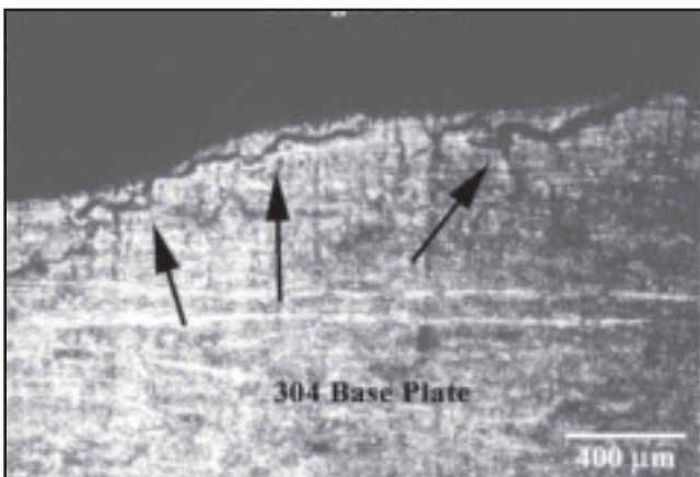
Fig. 7 — Toe cracking in the HAZ of the highest heat input stringer bead on the 304 base plate (Heat input: 136.6 kJ/in. 2 ).
