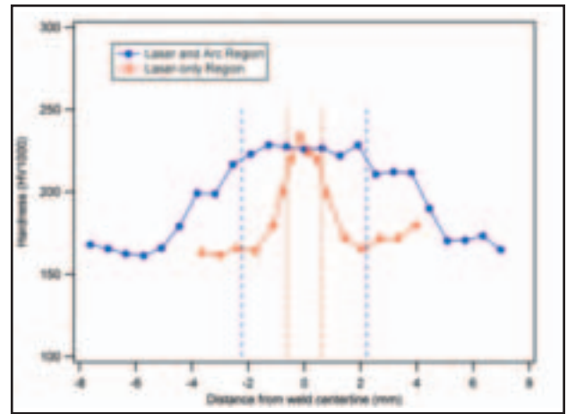
Fig. 5 — Hardness traverses through the two different regions of the two-part fusion zone partial penetration welds. Dotted lines show the location of the weld interface.
