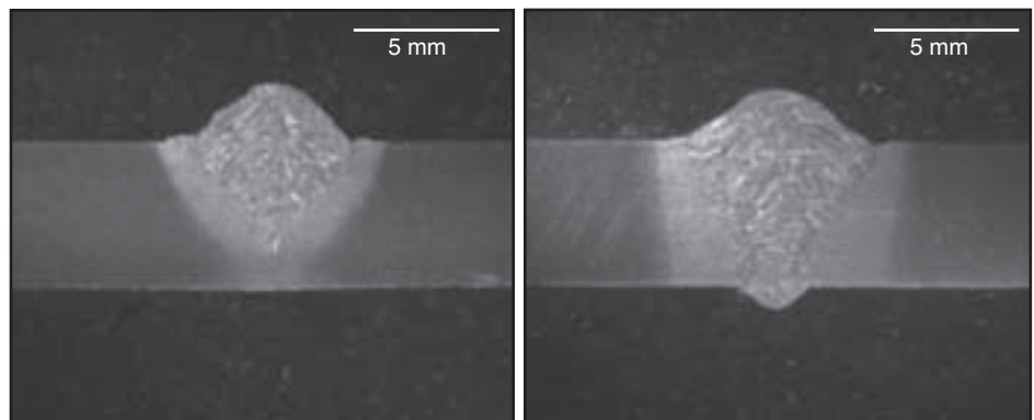
Fig. 7 — Macrographs showing the change in morphology associated with partial and complete penetration welds. Left — Partial penetration weld with a two-part fusion zone made with 4-kW laser power. Right — Full penetration weld with a uniform fusion zone made with 6-kW laser power.
