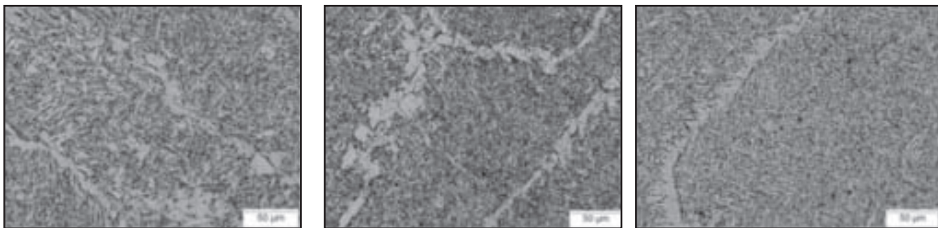
Fig. 18 — Micrographs showing the effect of laser-arc separation. From left, the laser arc separation is 4.5, 6.0, and 12.0 mm. Constants include laser power, 4.0 kW; and arc power, 8.5 kW.
