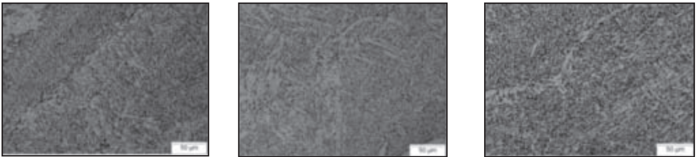
Fig. 16 — Micrographs showing the effect of arc power. From left, the arc power is 3.4, 6.3, and 8.5 kW. Constants include laser power, 8.0 kW, and laser-arc separation, 4.0 mm.
