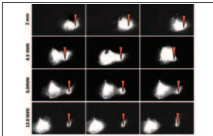
Fig. 20 — Selected high-speed video frames showing the differences caused by changing the laser-arc separation. Red triangles indicate the position of the laser beam.
