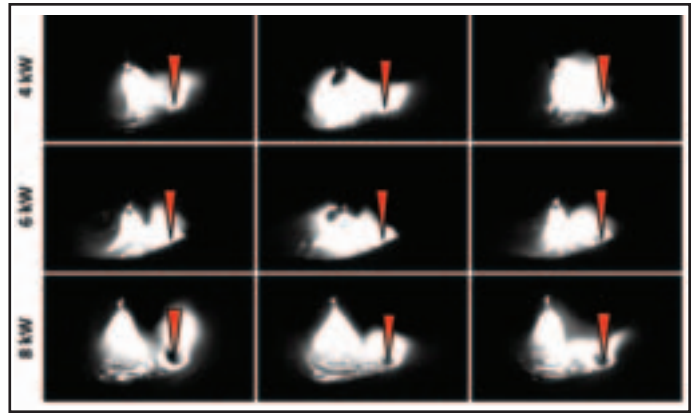
Fig. 22 — Selected high-speed video frames showing the differences caused by changing the laser power. Red triangles indicate the position of the laser beam.
