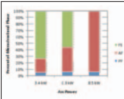
Fig. 17 — Weld metal microstructural content as a function of arc power. Laser power and laser-arc separation were constant at 8.0 kW and 4.0 mm, respectively.
