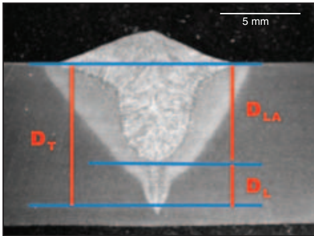
Fig. 9 — Schematic macrograph showing the penetration measurements of the laser and arc region, and the laser-only region.
