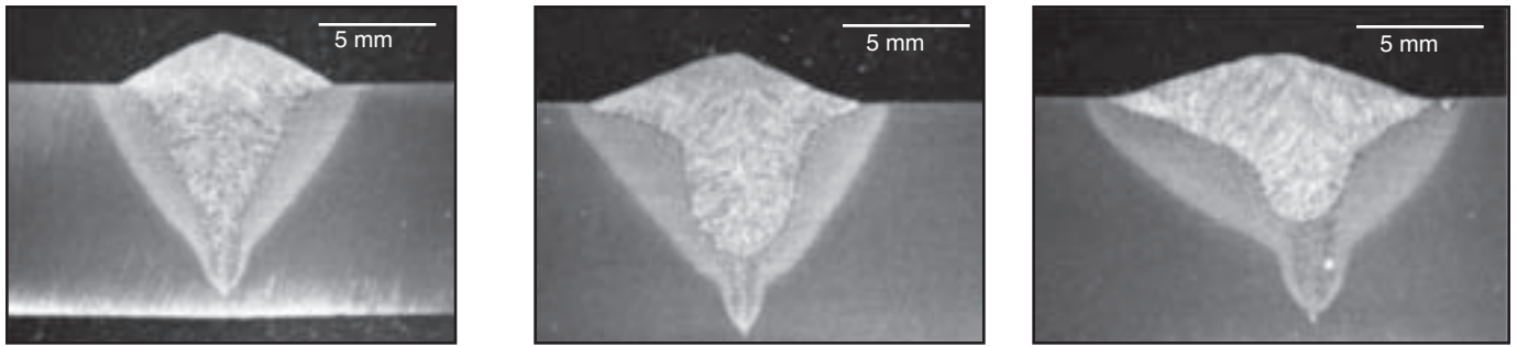
Fig. 8 — Macrographs showing the morphology changes due to the laser-arc separation in the partial penetration welds with a two-part fusion zone. From left, the laser-arc separation is 4.5, 6.0, and 12.0 mm. Laser power and arc power are constant for all welds at 8 and 8.5 kW, respectively.
