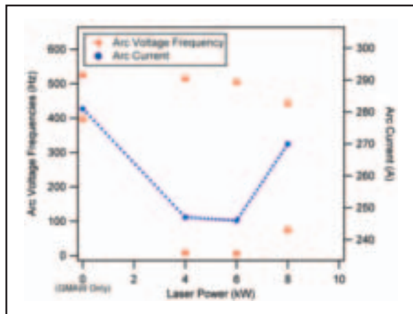
Fig. 23 — Major arc voltage frequencies and corresponding arc current as a function of laser power.
