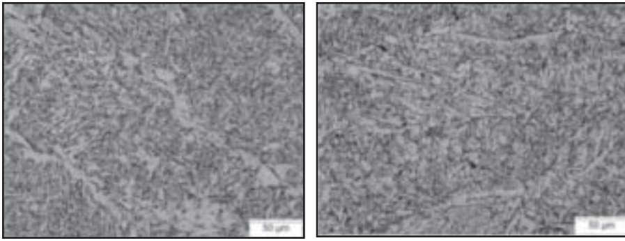
zFig. 14 — Micrographs showing the effect of laser power. From left, the laser power is 4 and 8 kW. Constants include arc power, 8.5 kW, and laser-arc separation, 4.5 mm.
