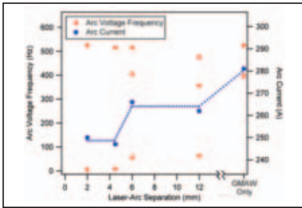
Fig. 21 — Major arc voltage frequencies and corresponding arc current as a function of laser-arc separation.
