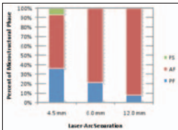
Fig. 19 — Weld metal microstructural content as a function of laser-arc separation. Laser power and arc power were constant at 4.0 and 8.5 kW, respectively.
