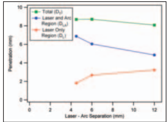
Fig. 10 — Total penetration and the penetration of the two distinct fusion zone regions as a function of the laser-arc separation in partial penetration bead-on-plate welds. Laser power and arc power are constant for all welds at 8 and 8.5 kW, respectively.
