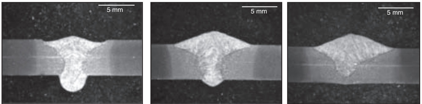
Fig. 11 — Macrographs showing the morphology changes due to the laser-arc separation in the welds with a uniform fusion zone. From left, the laser-arc separation is 4.5, 6.0, and 12.0 mm. Laser power and arc power are constant for all welds at 4 and 8.5 kW, respectively.
