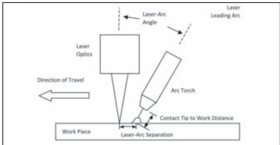
Fig. 1 — Schematic representation of the hybrid laser arc welding setup showing the direction of travel and critical dimensions.
