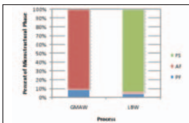
Fig. 13 — Weld metal microstructural content as process. The GMA weld was made with 8.5 kW of arc power, and the laser beam weld was made with 8 kW of laser power.
