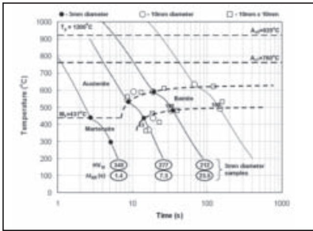
Fig. 1 — CCT diagram for X70 pipeline steel used in current experiments (Ref. 16).
