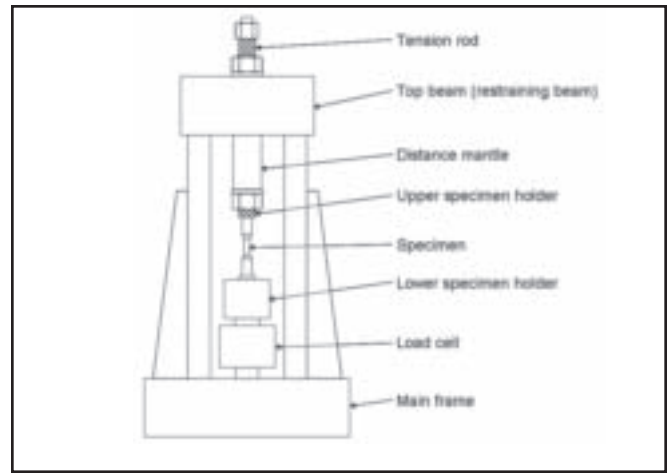
Fig. 3 — Schematic drawing of the Satoh test jig.
