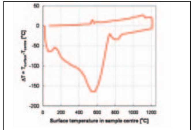
Fig. 9 — Modeled temperature difference between surface and center of the Satoh test sample. Conditions correspond to the case of a peak temperature of 1200°C.
