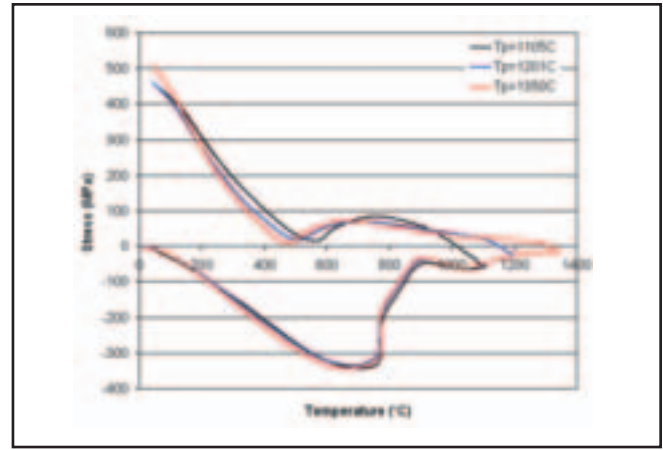
Fig. 7 — Effect of peak temperature on \sigma -T curves obtained for samples with cooling time \Delta t_{8/5} of around 10 s.
