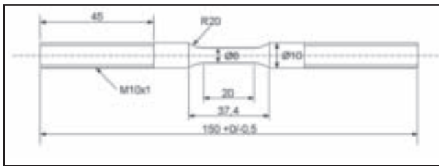
Fig. 2 — Specimen geometry for Satoh testing.
