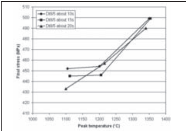
Fig. 8 — Effect of peak temperature on final stress in Satoh experiments.
