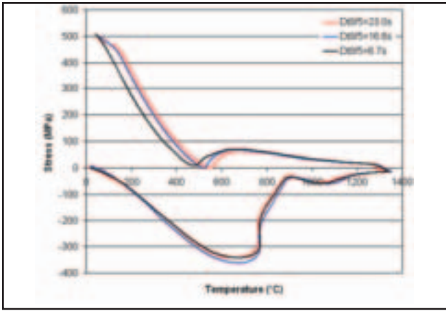
Fig. 6 — Effect of cooling rate on \sigma -T curves obtained for samples with peak temperatures of around 1350°C.
