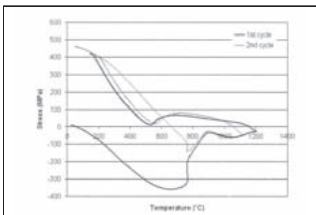
Fig. 12 — \sigma -T curve obtained for double thermal cycle experiment with first peak temperature of about 1200°C and second peak temperature of about 1000°C.
