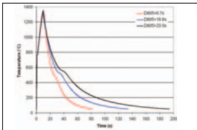
Fig. 4 — Measured temperature-time curves for samples with peak temperatures of around 1350°C.
