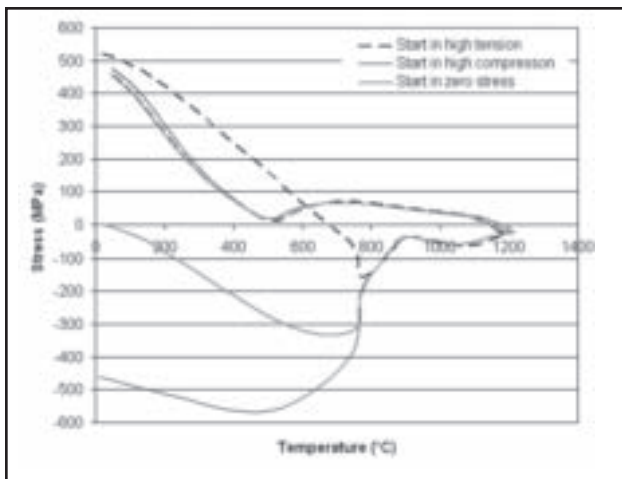
Fig. 10 — Effect of preloading on appearance of \sigma -T curve.
