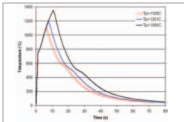
Fig. 5 — Measured temperature-time curves for samples with cooling time \Delta t_{8/5} of around 10 s.
