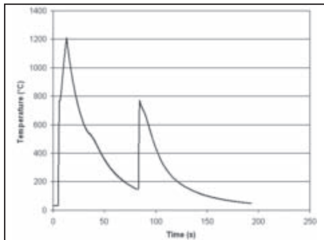
Fig. 11 — Typical measured temperature-time curve for double thermal cycle experiment.
