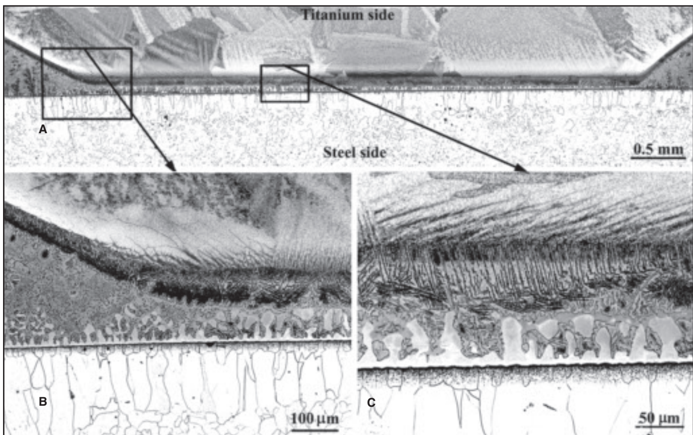
Fig. 2 — Microstructure of the joint brazed at 1000°C (1832°F). A — General view of the brazed joint; B — enlarged view of the fillet of the joint; C — enlarged view on the middle area of the joint.
