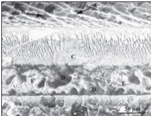
Fig. 3 — SEM image of the brazed joints at temperatures of 1000°C (1832°F).
