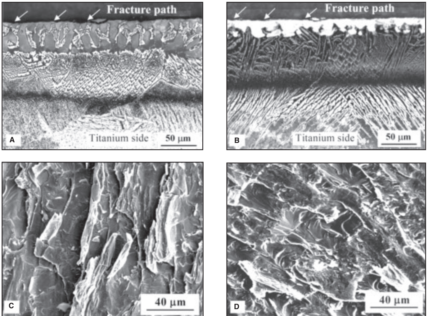
Fig. 8 — Cross-section fracture path and fracture morphology. A — Fracture path for a joint brazed at 1000°C (1832°F); B — fracture path for a joint brazed at 970°C (1778°F); C — fracture morphology for a joint brazed at 1000°C; D — fracture morphology for a joint brazed at 970°C.
