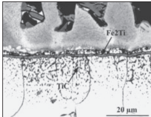
Fig. 4 — Microstructure at steel/copper interfacial area at a brazing temperature of 1000°C (1832°F).
