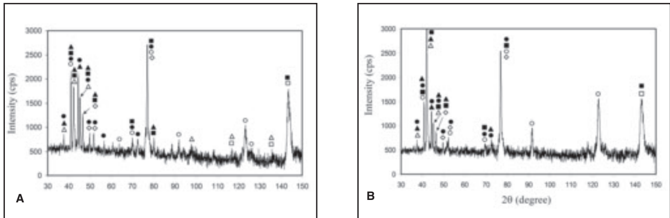
Fig. 9 — X-ray diffraction pattern of fracture surfaces of titanium side. A — Joint brazed at 1000°C (1832°F); B — joint brazed at 970°C (1778°F). Where diffraction lines from Ti, Fe, Cu, Mn, FeTi, Fe 2 Ti, and Ti x Mn are indicated by ○, △, □, ◇, ■, ▲, and ●, respectively.
