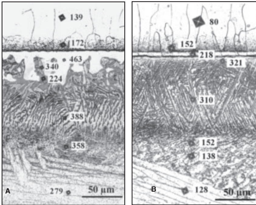
Fig. 6 — Hardness distribution along the brazed joints. A — Joint brazed at 1000°C (1832°F); B — joint brazed at 970°C (1778°F).
