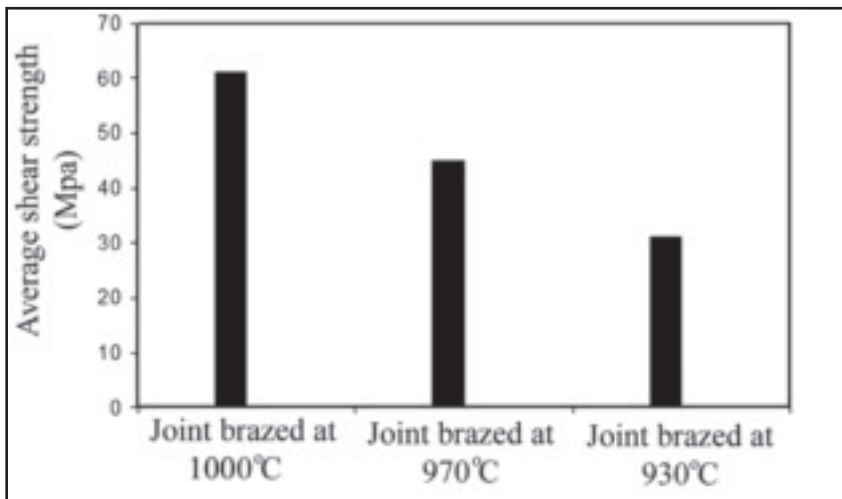
Fig. 7 — The average shear strengths of the joints at different brazing temperatures.
