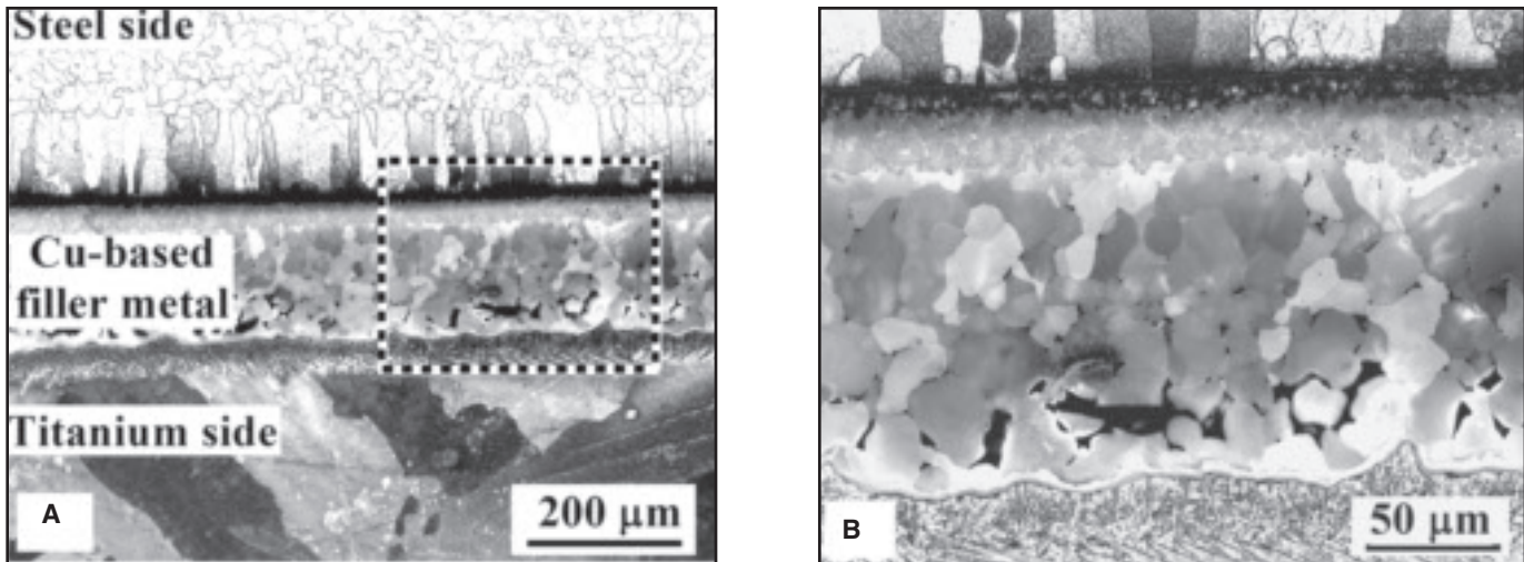
Fig. 1 — Microstructure of the joint brazed at 930°C (1706°F). A — General view of the microstructure; B — enlarged view of the brazed area.
