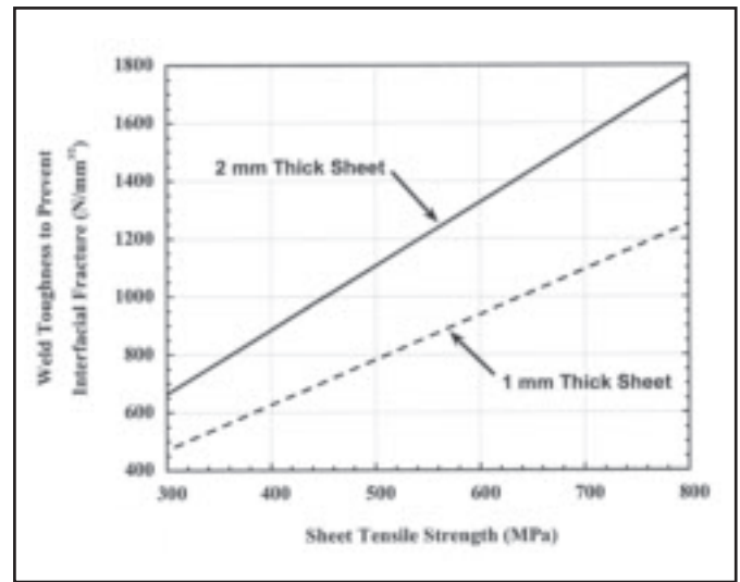
Fig. 15 — Predicted weld toughness required to avoid interfacial fracture in the shear-tension test as a function of sheet tensile strength for 1- and 2-mm-thick sheets.
