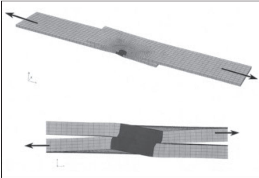
Fig. 8 — Mode-predicted deformation in the shear-tension test showing shear overload of the weld metal at the interface of the two sheets. Sheet thickness is 1.0 mm and button size is 4 mm.
