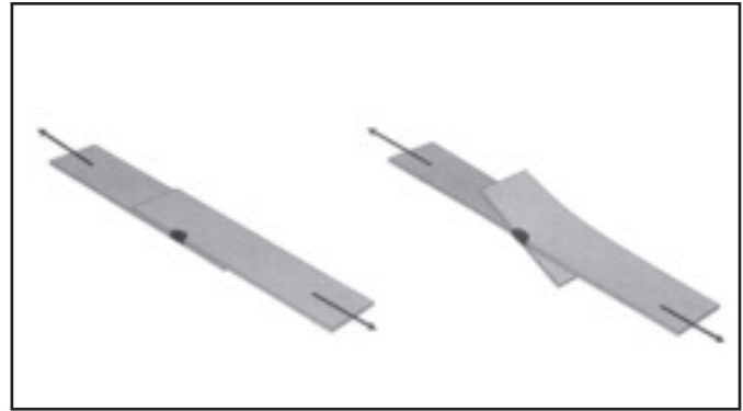
Fig. 2 — Sketches showing half sections of a shear-tension coupon before (left) and after (right) the application of load. Bending of the sample (shown in the right-side sketch) results from the offset of the sheets.
