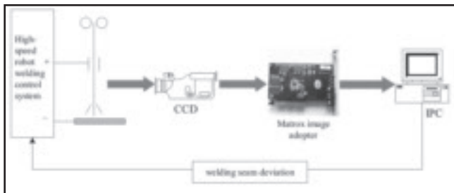
Fig. 1 — The developed intelligent weld tracking and control system.
