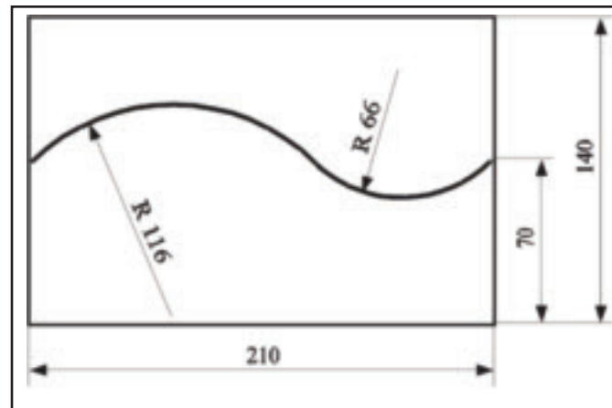
Fig. 6 — The geometry chart of the weld joint.
