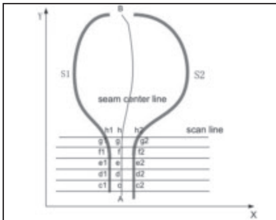
Fig. 5 — The method for detecting welding joint center.
