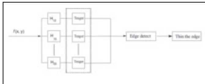
Fig. 3 — The image edge detecting flow with M-band wavelet transform.
