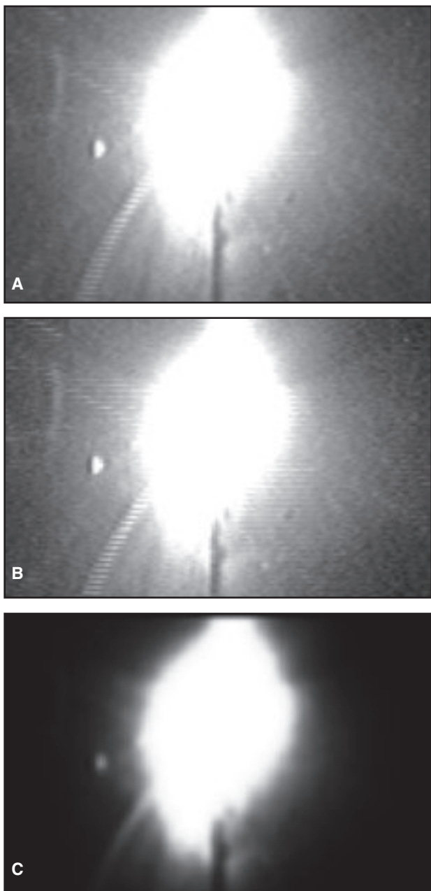
Fig. 2 — Result of image preprocessing: filtering and squaring. A — The original welding image; B — the result after median filtering; C — the result after filtering and squaring.
