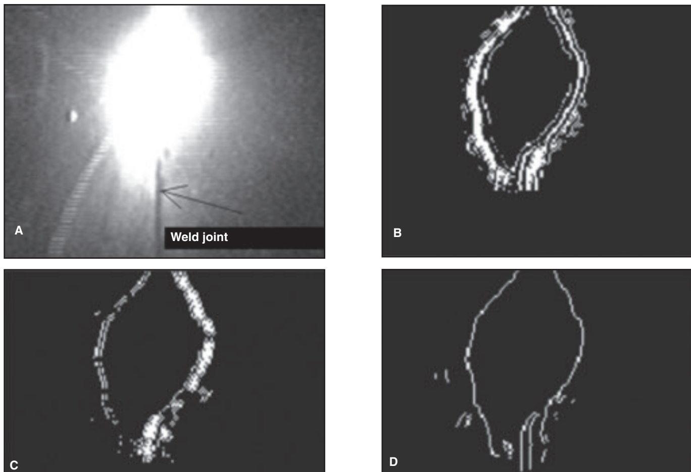
Fig. 4 — The results of molten pool image edge detection with M-band wavelet transform. A — Molten weld pool; B — horizontal result; C — vertical result; D — synthetic result.
