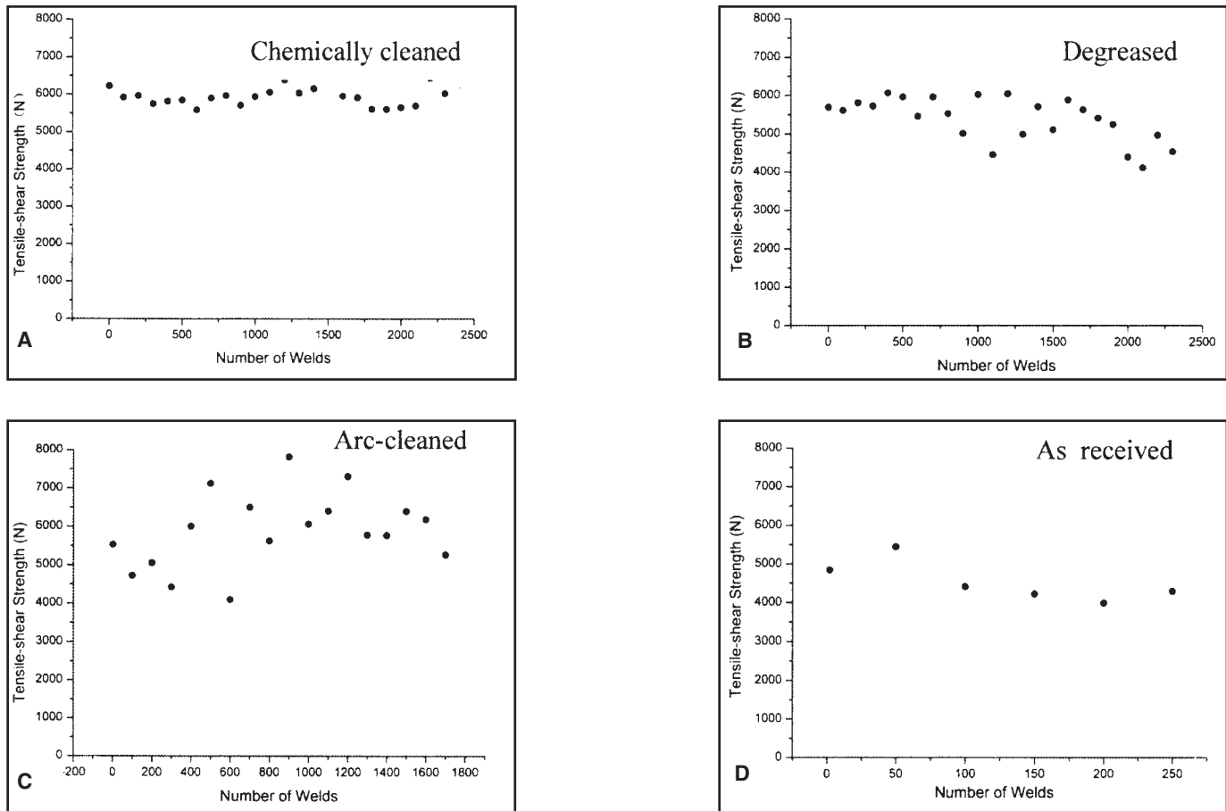
Fig. 9 — Tensile-shear strengths of welds. A — Chemically cleaned; B — degreased; C — electric-arc cleaned; D — untreated sheets, taken during electrode life tests.
