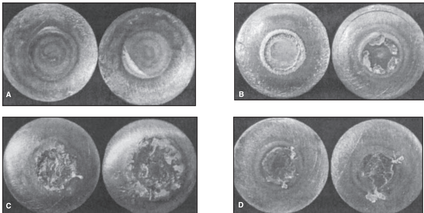
Fig. 7 — Electrode surface morphology after life tests. A — Chemically cleaned; B — degreased; C — electric-arc cleaned; D — untreated aluminum sheets. The electrodes on the left side are from the lower arm of the welding machine (negative), and those on the right side are from the upper arm (positive).
