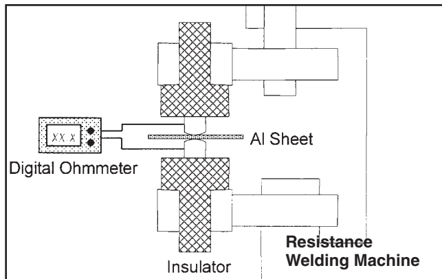
Fig. 1 — Setup for contact resistance measurement.
