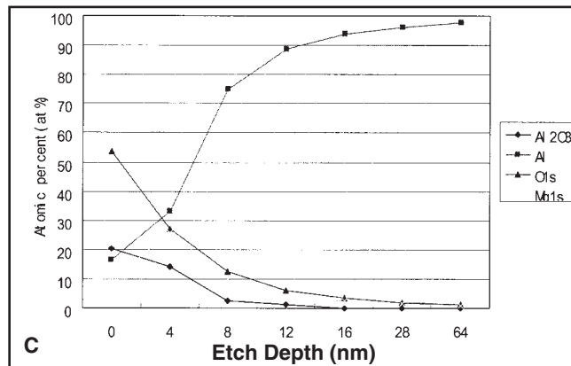
Fig. 2 — Profiles of atomic-percent of various elements in the surface layers after cleaning. A — Degreasing; B — chemical cleaning; C — electric-arc cleaning.
