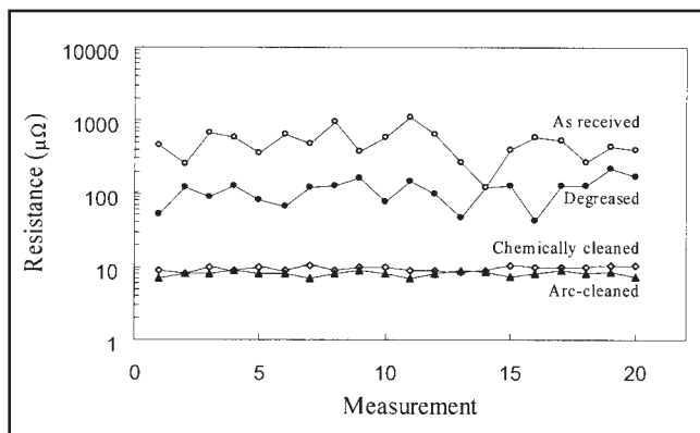
Fig. 3 — Resistance measurement of various surface conditions.
