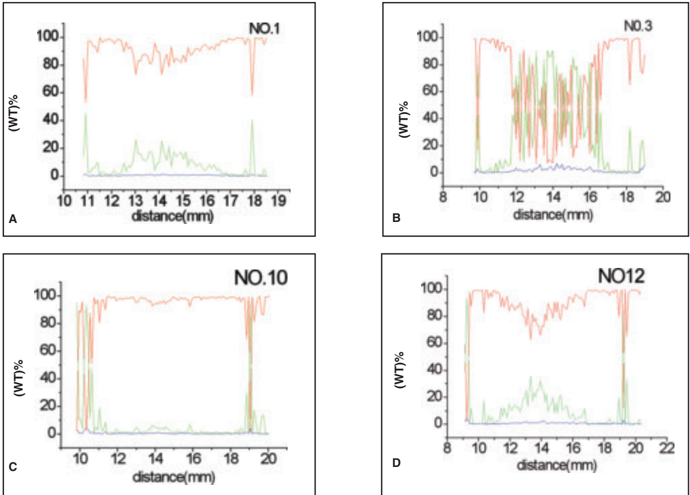
Fig. 5 — Composition profiles of electrode surfaces after 60 welds using the schedules of A — F = 4.5 \text{ kN} , \tau = 60 \text{ ms} ; B — F = 4.5 \text{ kN} , \tau = 180 \text{ ms} ; C — F = 9.0 \text{ kN} , \tau = 60 \text{ ms} ; D — F = 9.0 \text{ kN} , \tau = 180 \text{ ms} . The red line is for Cu, green is for Al, and blue is for Mg.
