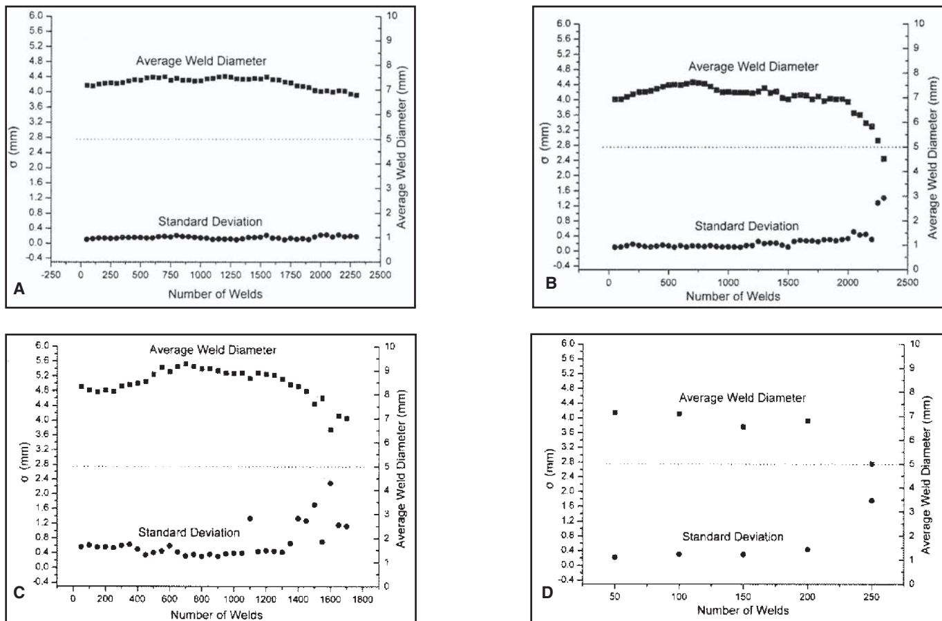
Fig. 8 — Average diameters and standard deviations of welds. A — Chemical cleaning; B — degreasing; C — electric-arc cleaning methods; D — untreated sheets.
