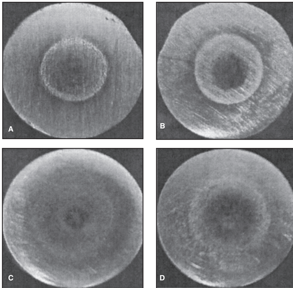
Fig. 4 — Electrode surfaces after making 60 welds on sheets of different surface conditions. A — Chemically cleaned; B — degreased; C — electric-arc cleaned; D — untreated.
