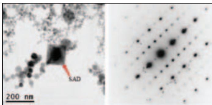
Fig. 10 — Large, square Mn:Fe_3O_4 fume particle from high-Mn FCAW. [013] zone axis.
