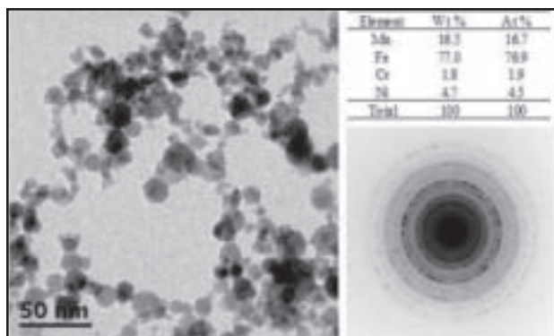
Fig. 9 — Small particle agglomerate from high-Mn FCAW fume that shows Fe_3O_4 type crystal structure. Oxygen was not included in this analysis.
