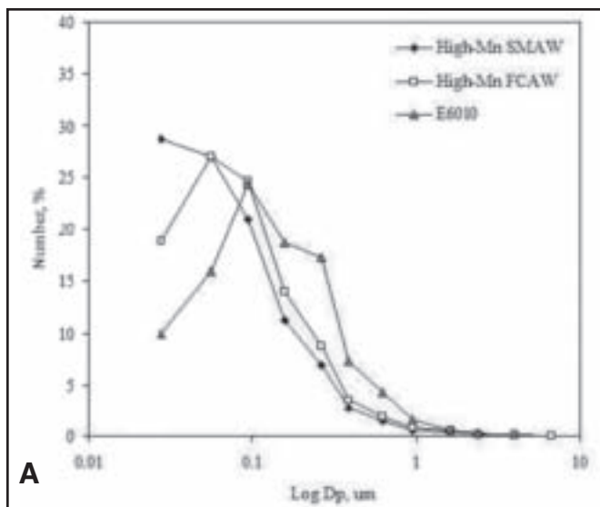
Fig. 1 — Distributions of high-Mn consumable fume and E6010 fume. A — Number; B — mass.
