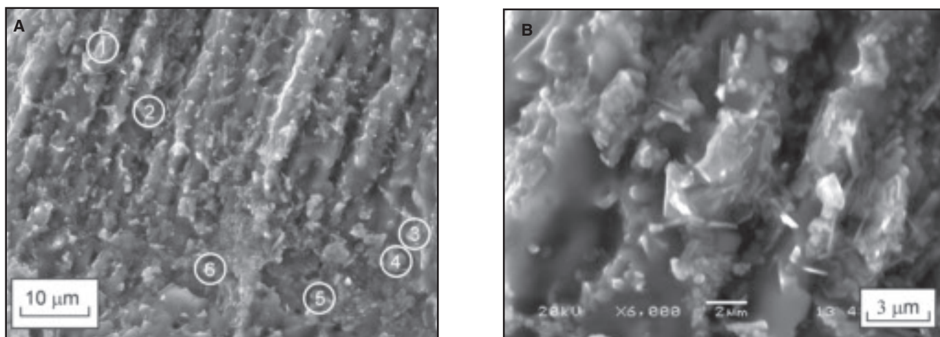
Fig. 15 — SEM photographs of crack surfaces in welds made using a ramp-down pulse shape with peak power density of the main welding sector of 11.5 GW/m 2 and ramp-down gradient of 3 kW/s: A — Overall crack surface; B — higher magnification for area of interest in ① in A.
