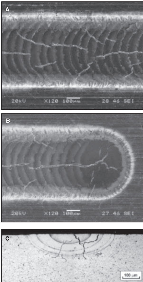
Fig. 6 — Severe solidification cracking in a weld made with a rectangular pulse shape with a peak power density of 11.5 \text{ GW/m}^2 : A — Weld bead during steady welding; B — end of weld bead with crater cracking; and C — transverse section.
