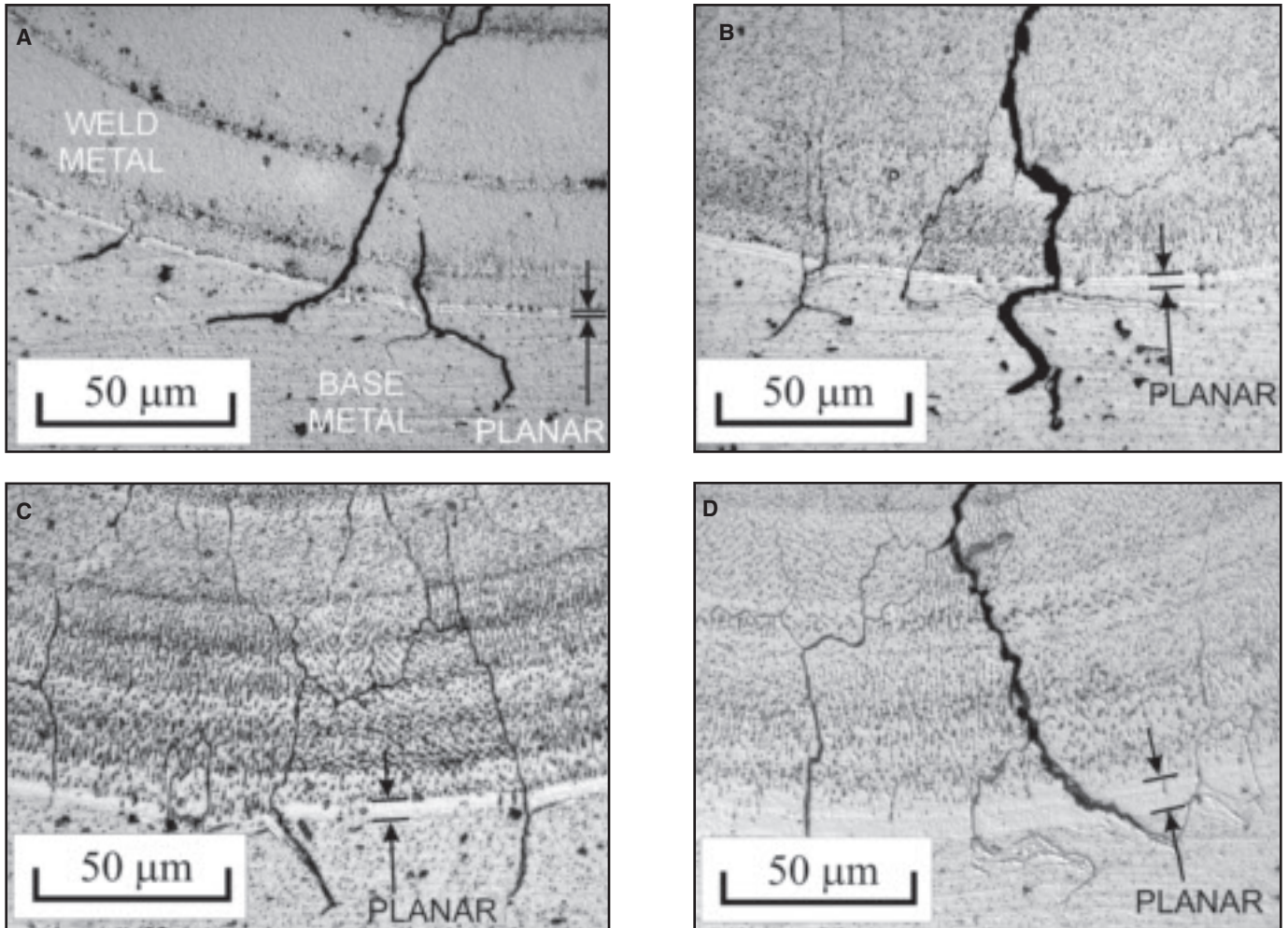
Fig. 13 — Effect of ramp-down gradient on solidification morphologies of welds made using a main welding sector peak power density of 11.4 \text{ GW/m}^2 and the following: A — A rectangular pulse shape and pulses with ramp-down gradients of — B — 420 \text{ kW/s} ; C — 100 \text{ kW/s} ; and D — 36 \text{ kW/s} .
