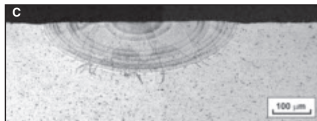
Fig. 8 — A sound weld made using a ramp-down pulse shape with main welding sector peak power density of 11.5 \text{ GW/m}^2 and ramp-down gradient of 100 \text{ kW/s} : A — Weld bead during steady welding; B — end of weld bead with crater area; and C — transverse section.
