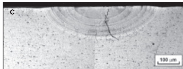
Fig. 9 — Intermittent solidification cracking in a weld made using a ramp-down pulse shape with main welding sector peak power density of 11.5 \text{ GW/m}^2 and ramp-down gradient of 36 \text{ kW/s} : A — weld bead during steady welding; B — end of weld bead with crater cracking; and C — transverse section.
