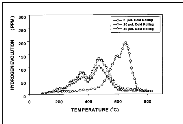
Fig. 12 — Thermal desorption analysis of stress-induced, dual-phase steel after gaseous hydrogen charging.
