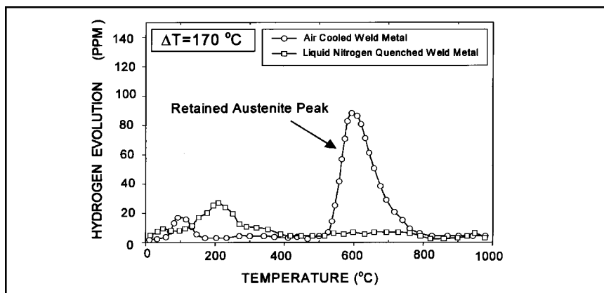
Fig. 7 — Thermal desorption analysis of hydrogen-charged HSLA steel weld metal.
