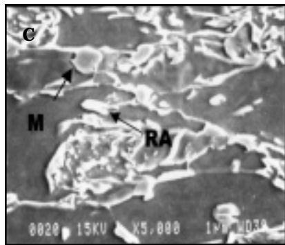
Fig. 10 — The measured retained austenite content. A — As function of tensile strain at room temperature; B — quenching temperature; C — scanning electron micrograph of steel structure deformed to a tensile strain of 10% at room temperature (M: martensite, RA: retained austenite).
