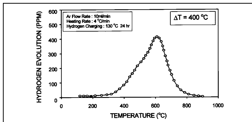
Fig. 3 — Thermal desorption analysis of hydrogen-charged super duplex stainless steel sample.
