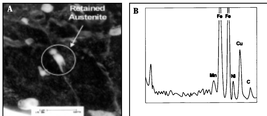
Fig. 9 — HSLA weld metal, which contains 4 vol-% retained austenite. A — TEM microstructure; B — EDS analysis on retained austenite particle.
