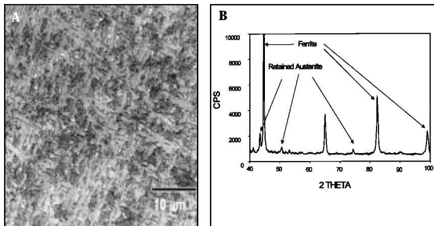
Fig. 8 — A — Optical microstructure of HSLA weld metal, which contains 4 vol-% retained austenite; B — X-ray analysis of HSLA steel weld metal, which contains 4 vol-% retained austenite.
