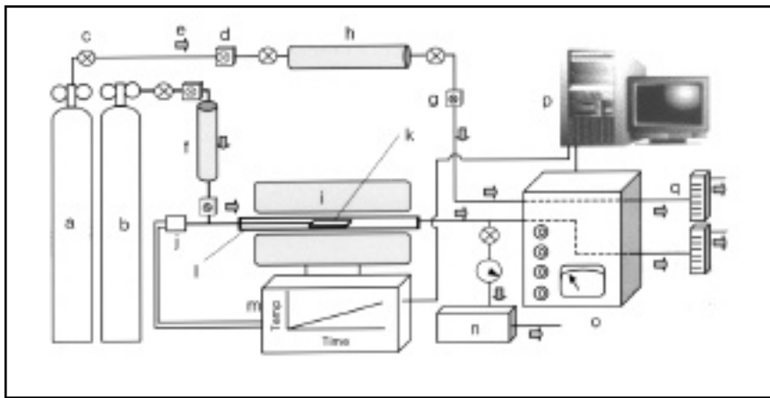
Fig. 1 — Hydrogen thermal desorption analysis apparatus. a — reference gas cylinder (argon); b — carrier gas cylinder (argon); c — valve; d — pressure gauge; e — gas flow direction; f — oxygen trap; g — flow gauge; h — moisture trap; i — furnace; j — thermocouple; k — sample; l — fused silica tube; m — furnace controller; n — vacuum pump; o — gas chromatograph; p — computerized data acquisition system; q — flow meter.
