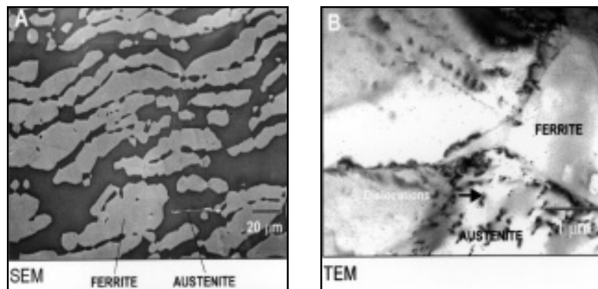
Fig. 4 — Microstructure of super duplex stainless steel. A — SEM; B — TEM.
