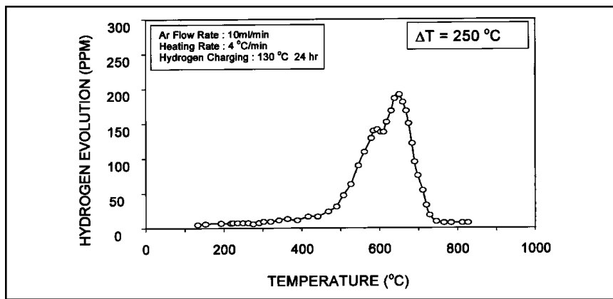
Fig. 5 — Thermal desorption analysis of a hydrogen-charged dual-phase steel sample.
