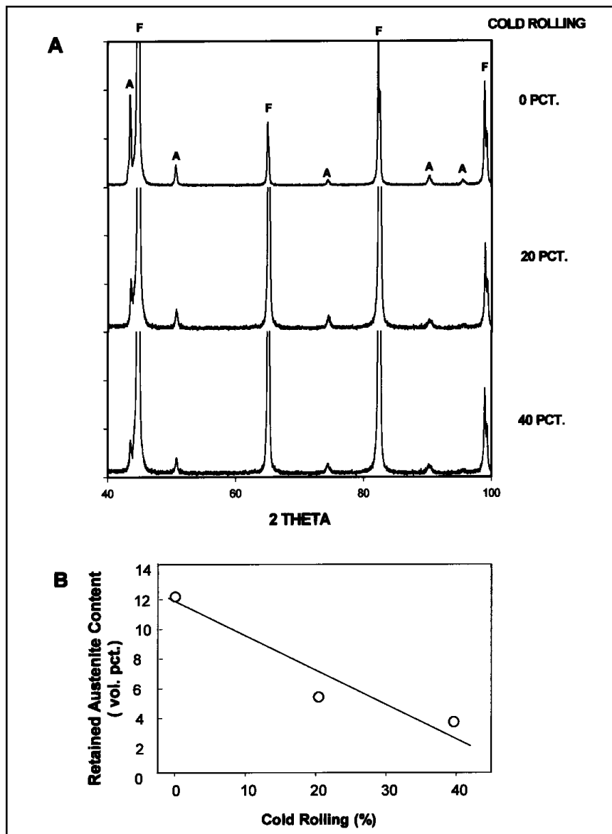
Fig. 11 — A — XRD result for 20 and 40% cold-rolled dual-phase steel (A — Austenite Peak and F — Ferrite Peak); B — the measured retained austenite content as function of cold rolling at room temperature.
