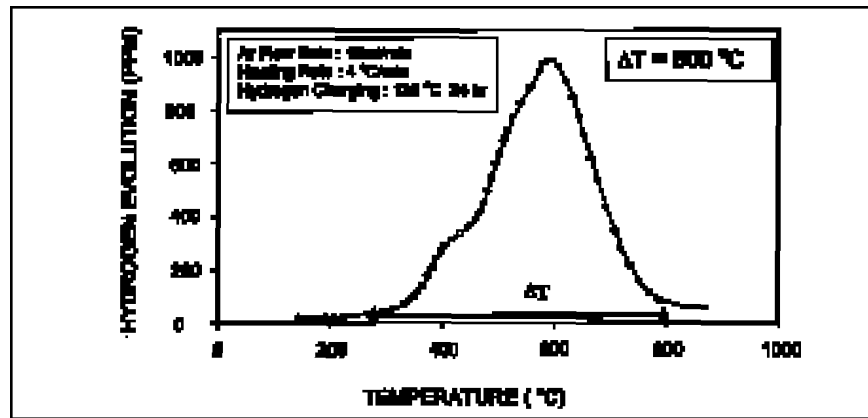
Fig. 2 — Typical thermal desorption analysis result from a hydrogen-charged AISI type 304 stainless steel sample.
