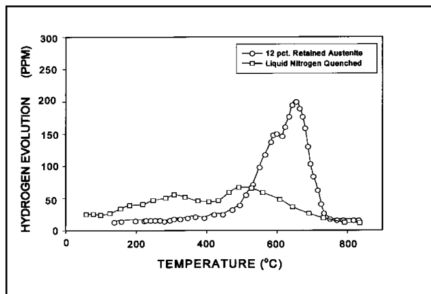
Fig. 13 — Thermal desorption analysis for dual-phase steel that is quenched in liquid nitrogen after charging.
