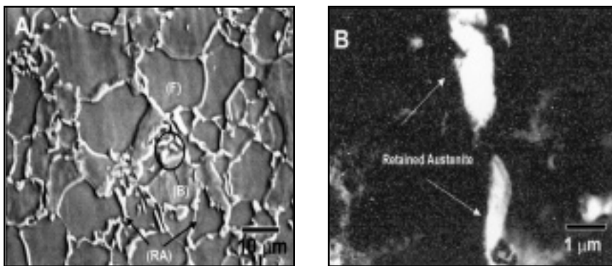
Fig. 6 — A — SEM microstructure of intercritically heat treated steel, which contains 12 vol-% retained austenite; B — detail of the area shown in A; (RA) Retained Austenite, (F) Ferrite, (B) Bainite.
