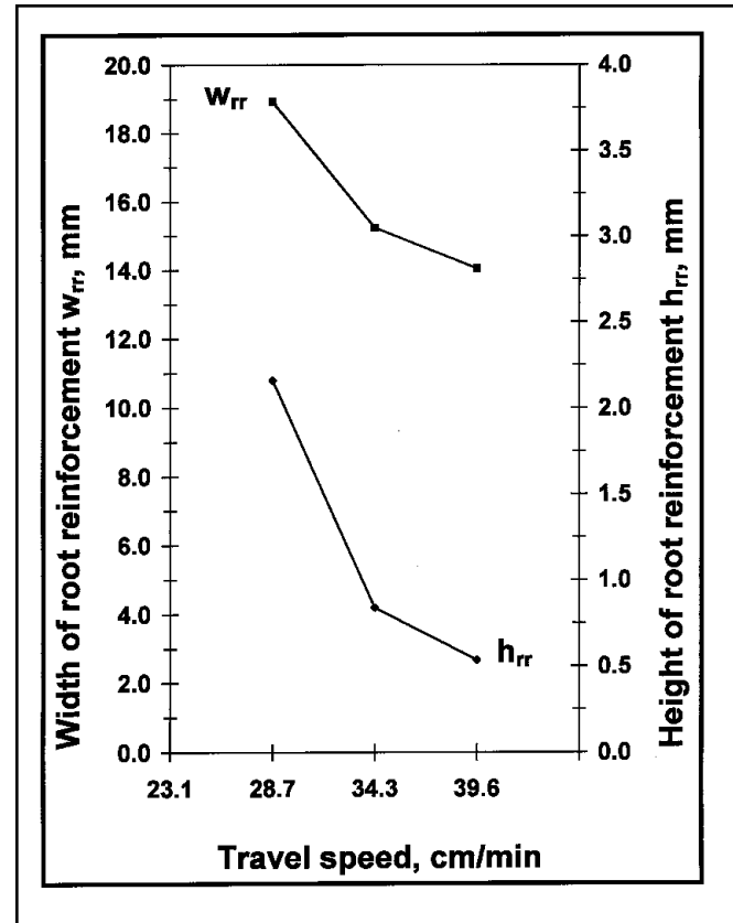
Fig. 11 — Effect of travel speed on geometry of the root reinforcement. h_{rr} = height of the root reinforcement; w_{rr} = width of the root reinforcement.
