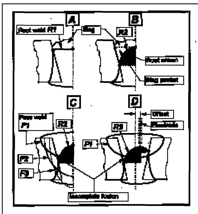
Fig. 2 — Relationships between the shape of the root bead and defect formation. A — Desirable (flat) shape of the root bead; B — undesirable crowned shape of the root bead and the resulting slag pockets; C — incomplete fusion in the fill weld due to slag pockets; D — slag pocket developed due to offset of the electrode.
