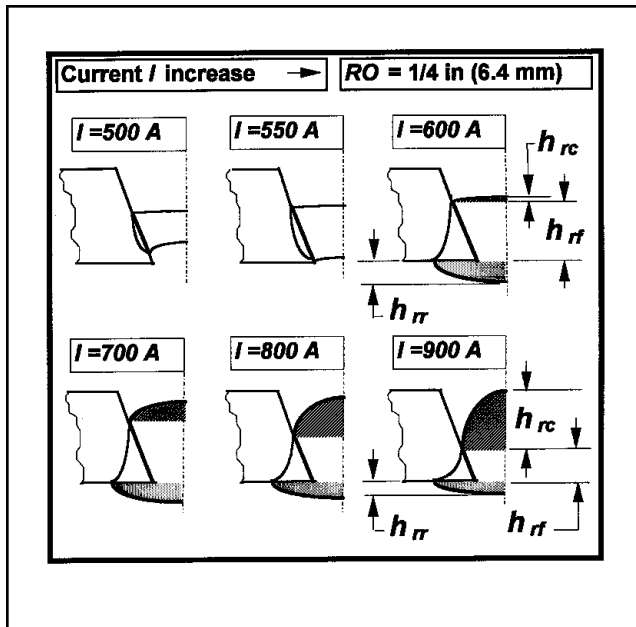
Fig. 6 — Relationships between the shape of the root bead and the current.
