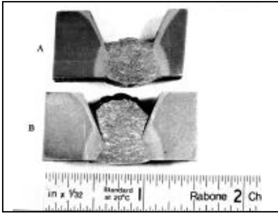
Fig. 5 — Cross sections of the root beads deposited at different currents. A — I = 600 A; B — I = 1000 A.
