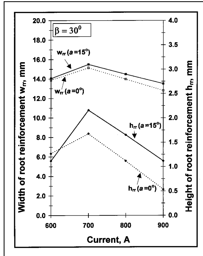
Fig. 13 — Effect of electrode inclination ( ) on geometry of the root reinforcement. h_{rr} = height of the root reinforcement; w_{rr} = width of the root reinforcement.
