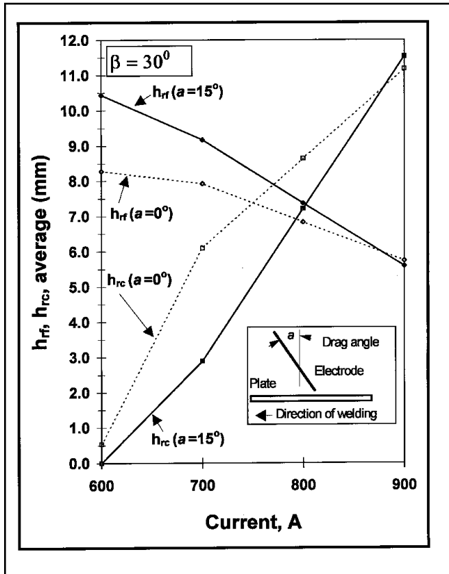
Fig. 12 — Effect of electrode inclination ( ) on fusion characteristics of the root bead. h_{rf} = height of root fusion; h_{rc} = height of the root crown (slag pocket).
