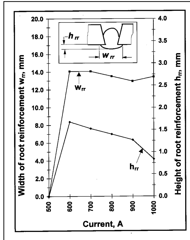
Fig. 9 — Effect of current on geometry of the root reinforcement. h_{rr} = height of the root reinforcement; w_{rr} = width of the root.
