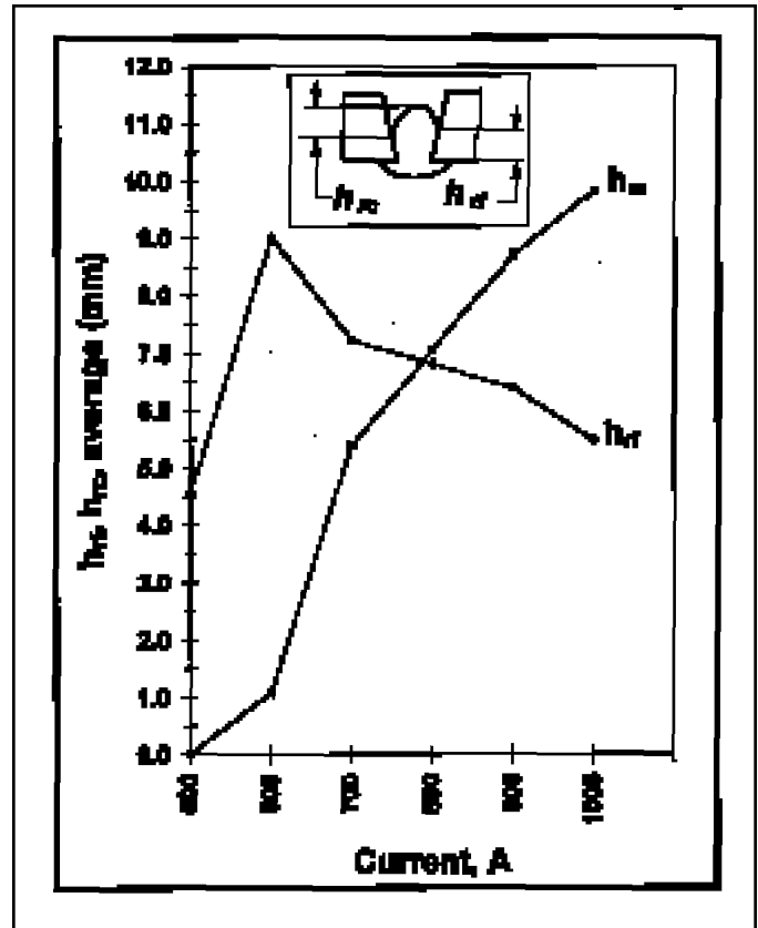
Fig. 7 — Effect of current on fusion characteristics of the root bead. h_{rf} = height of root fusion; h_{rc} = height of the root crown (slag pocket).
