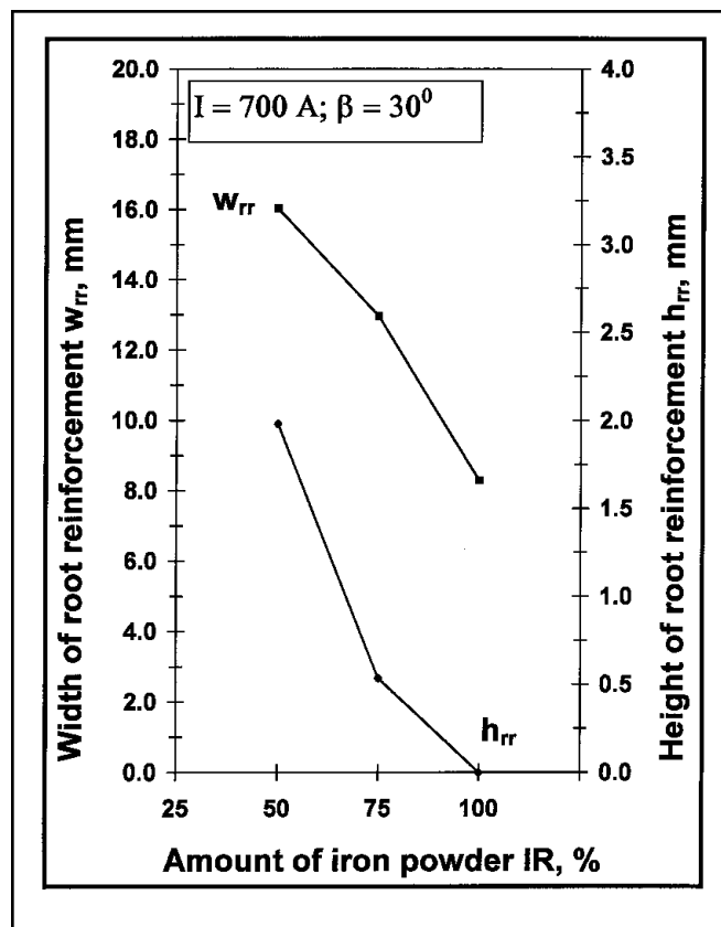
Fig. 15 — Effect of iron powder on geometry of the root reinforcement. h_{rr} = height of the root reinforcement; w_{rr} = width of the root reinforcement.
