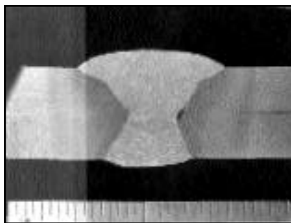
Fig. 3 — Incomplete fusion in the fill weld due to a slag pocket on one side of the root bead.
