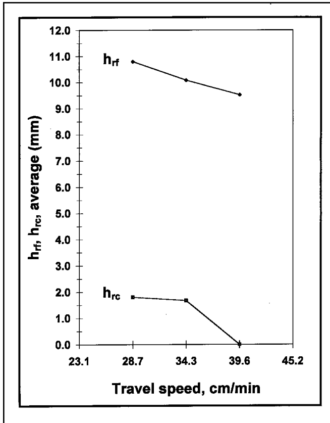
Fig. 10 — Effect of travel speed on fusion characteristics of the root bead. h_{rf} = height of root fusion; h_{rc} = height of the root crown (slag pocket).
