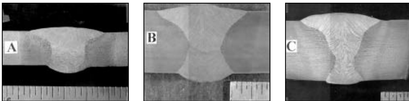
Fig. 1 — Welds completed by one-pass, two-electrode, one-sided MRF welding in plates of various thicknesses ( T ) assembled with large root openings ( RO ). A — T = 9.5 mm and RO = 4.8 mm; B — T = 17.5 mm and RO = 6.4 mm; C — T = 25.4 mm and RO = 6.4 mm. (Scale: 1 division = \frac{1}{16} in. = 1.6 mm).
