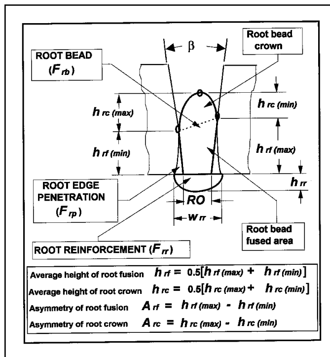
Fig. 4 — Characteristic areas and dimensions of the root bead.
