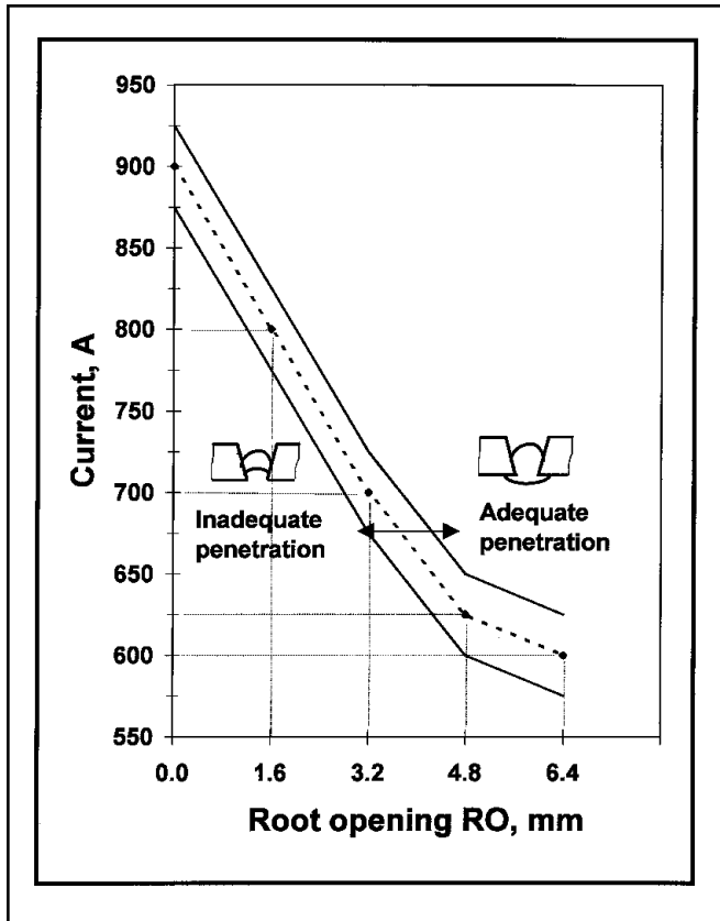
Fig. 8 — The current required for adequate root edge penetration at various root openings.
