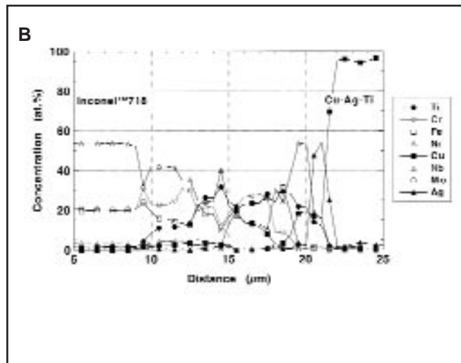
Fig. 12 — EMPA traces for the Inconel™ 718/Ag-Cu-Ti brazed joints. A — After aging at 150°C (302°F) for 100 days; B — after aging at 575°C (1067°F) for 300 days.
