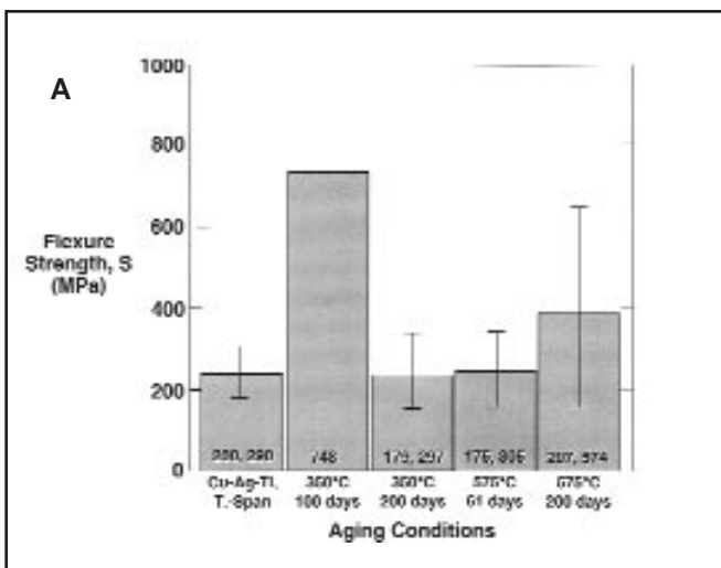
Fig. 13 — A — Bar chart of mean strength values for the aged Thermo-Span™/Ag-Cu-Ti brazed joints; B — bar chart of mean strength values for the aged Inconel™ 718/Ag-Cu-Ti brazed joints.
