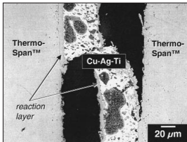
Fig. 15 — Optical micrograph of the fracture path in a Thermo-Span™/Ag-Cu-Ti specimen that was aged at 575°C (1067°F) for 200 days prior to testing.
