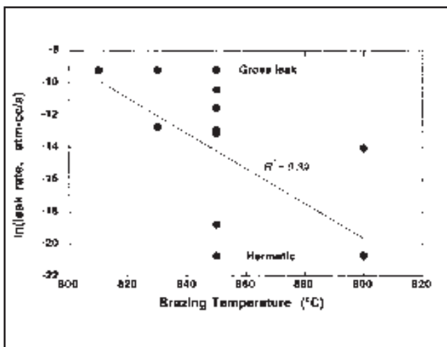
Fig. 3 — Logarithm (natural) of the leak rate as a function of brazing temperature for a brazing time of 5 min.
