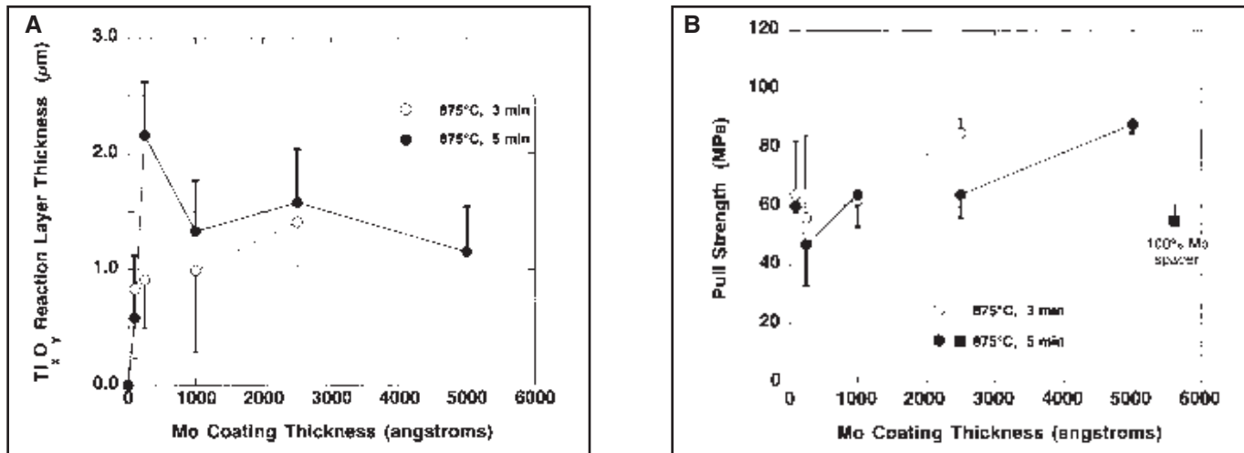
Fig. 20 — A — Graph of the Ti_xO_y reaction layer thickness as a function of the molybdenum coating thickness for the 875°C, 3- and 5-min brazing processes; B — pull strength as a function of the molybdenum coating thickness for the 875°C, 3- and 5-min brazing processes. The 100% molybdenum spacer data have been included in both plots.
