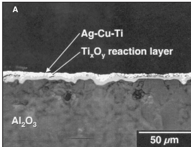
Fig. 10 — Optical micrographs of cross sections showing details of the Ag-Cu-Ti/Al 2 O 3 failure mode from pull tested braze joints made with the 100% molybdenum spacer. A — Fracture in the filler metal near the Ag-Cu-Ti/Ti x O y interface; B — fracture at the Ti x O y /Al 2 O 3 interface. The sample was brazed at 850°C for 5 min.
