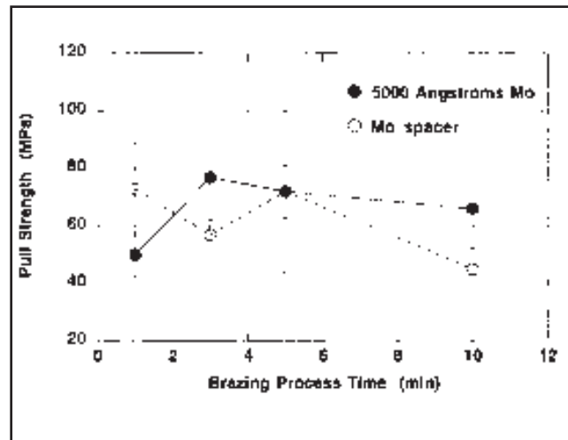
Fig. 7 — Pull strength as a function of brazing time for a 850°C brazing temperature. Specimens were assembled with a 5000-Å Mo-coated, Fe-29Ni-17Co spacer or with the 100% molybdenum spacer.
