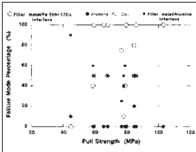
Fig. 8 — Failure mode as a function of pull strength for all samples having the 5000-Å molybdenum-coated Fe-29Ni-17Co spacer. Samples were brazed at 850 and 875°C.
