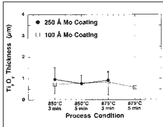
Fig. 17 — The Ti x O y reaction layer thickness as a function of the brazing process for specimens assembled with Fe-29Ni-17Co spacers having a 250- or 100-Å molybdenum barrier layer.
