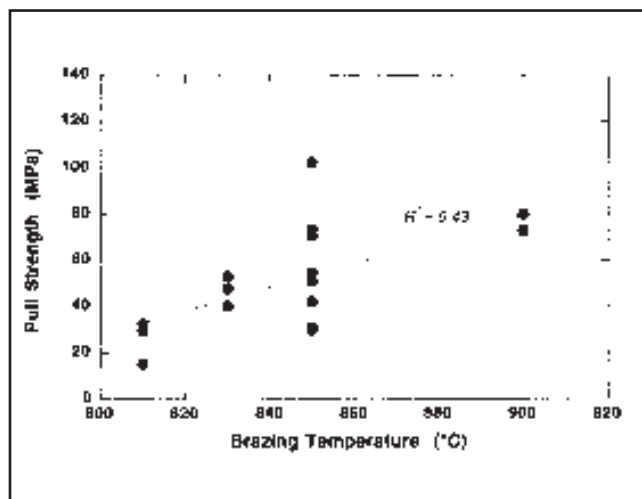
Fig. 4 — Joint pull strength as a function of brazing temperature for a brazing time of 5 min.
