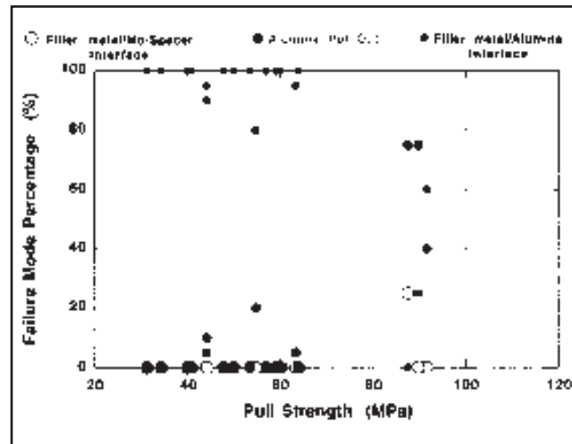
Fig. 9 — Failure mode as a function of pull strength for all samples having the 100% molybdenum spacer. Samples were brazed at 850 and 875°C.
