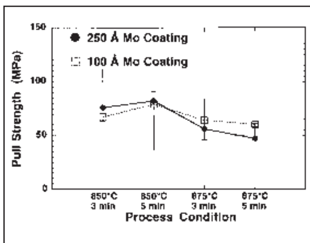
Fig. 18 — Pull strength as a function of process conditions for specimens brazed with 250- or 100-Å molybdenum-coated Fe-29Ni-17Co spacers.
