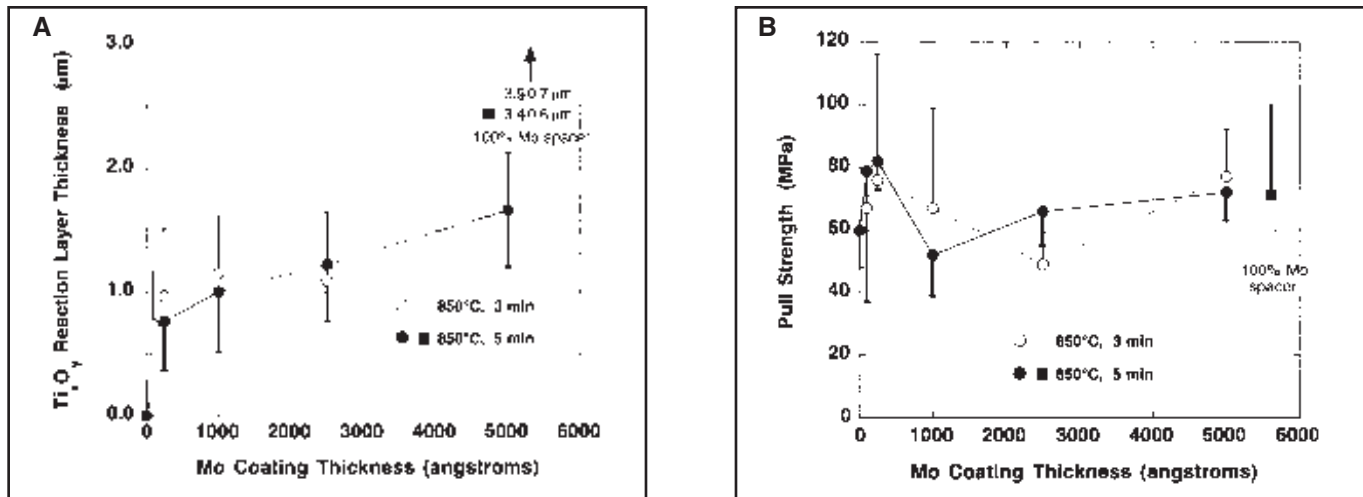
Fig. 19 — A — Graph of the Ti x O y reaction layer thickness as a function of the molybdenum coating thickness for the 850°C, 3- and 5-min brazing processes; B — pull strength as a function of the molybdenum coating thickness for the 850°C, 3- and 5-min brazing processes. The 100% molybdenum spacer data have been included in both plots.
