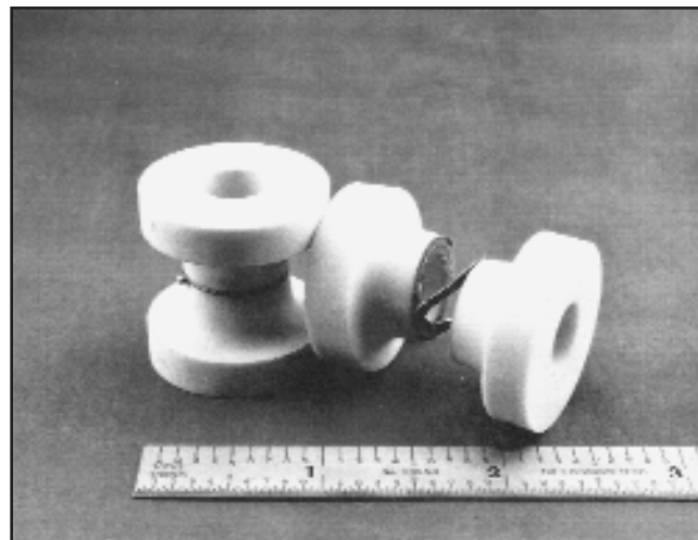
Fig. 2 — Geometry of the ASTM-F19 tensile button specimen. The location of the spacer and brazed joints are shown in the tested sample on the right-hand side of the photograph.
