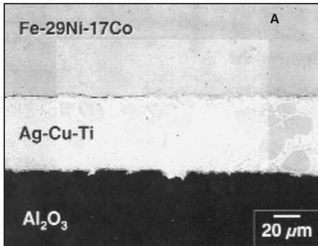
Fig. 5 — Optical micrographs of the following: A — the entire braze joint; B — the filler metal/ Al_2O_3 interface from the test specimen having a 5000-Å Mo layer on the Fe-29Ni-17Co spacer. The process conditions were 850°C and 5 min.
