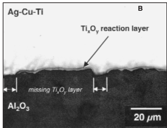
Fig. 15 — Optical micrograph of the joint fabricated with the 250-Å molybdenum-coated Fe-29Ni-17Co spacer, viewing specifically; A — the Ag-Cu-Ti/(Mo)Fe-29Ni-17Co interface; B — the Ag-Cu-Ti/Al 2 O 3 interface. Gaps in the layer are indicated by arrows and brackets. The brazing conditions were 850°C for 5 min.
