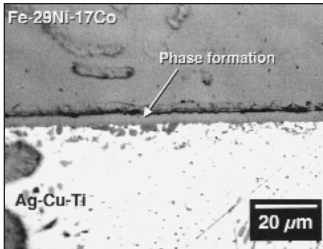
Fig. 16 — Optical micrograph of the Ag-Cu-Ti/(Mo)Fe-29Ni-17Co interface in a specimen assembled with the 100-Å molybdenum-coated Fe-29Ni-17Co spacer. Brazing conditions were 850°C for 5 min.
