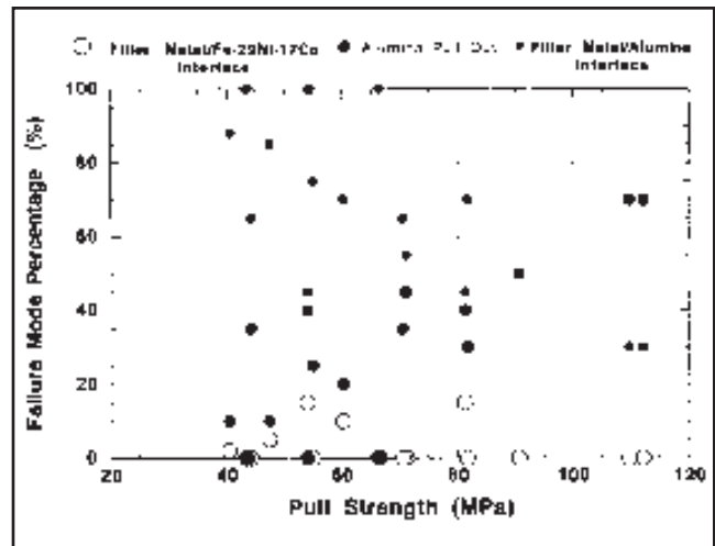
Fig. 14 — Failure mode as a function of pull strength for specimens having the 2500-Å molybdenum-coated Fe-29Ni-17Co spacer and which were brazed at 850 and 875°C.
