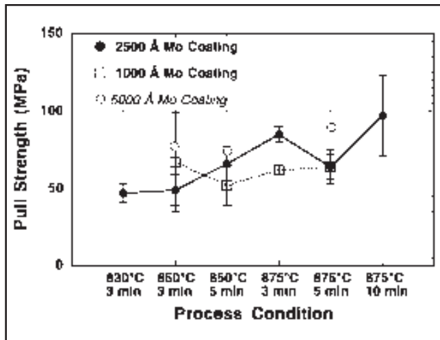
Fig. 13 — Pull strength as a function of brazing conditions for specimens assembled with 2500- and 1000-Å molybdenum-coated Fe-29Ni-17Co spacers.
