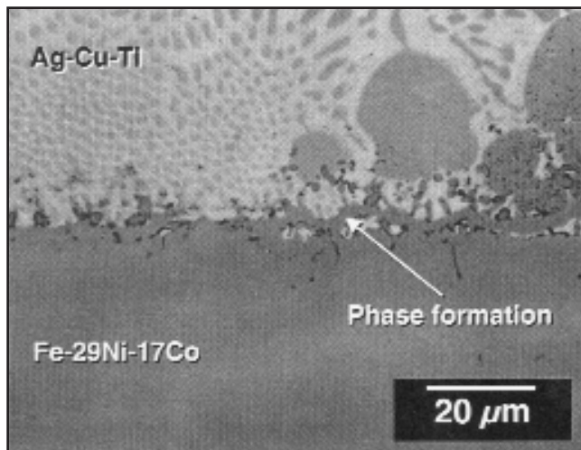
Fig. 11 — Optical micrograph showing a cross section at the Ag-Cu-Ti/(Mo) Fe-29Ni-17Co interface of the joint made with the Fe-29Ni-17Co spacer having a 1000-Å molybdenum coating. The joint was brazed at 850°C for 5 min.
