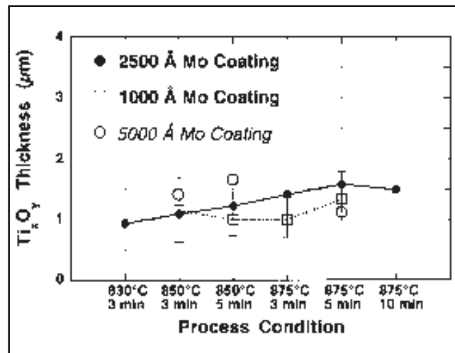
Fig. 12 — The Ti x O y reaction layer thickness as a function of the brazing process for specimens assembled with Fe-29Ni-17Co spacers having a 2500- or 1000-Å molybdenum barrier layer.
