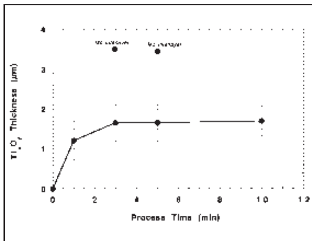
Fig. 6 — The Ti_xO_y reaction layer thickness as a function of brazing time for Fe-29Ni-17Co spacers coated with 5000 Å of molybdenum. The brazing temperature was 850°C. Corresponding data for the 100% molybdenum spacer have been included.
