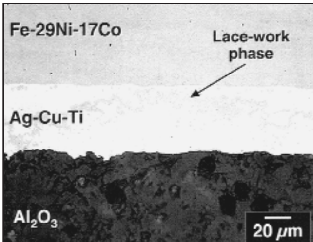
Fig. 1 — Optical micrograph of an Al_2O_3/Al_2O_3 joint made with a Fe-29Ni-17Co interlayer between it and using the Ag-Cu-Ti filler metal. The brazing conditions were 850°C and 5 min.
