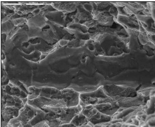
Fig. 9 — Fracture surface showing a kissing bond in a transverse weld in AA6082 (at higher magnification). The kissing bond is in the plane of the picture.
