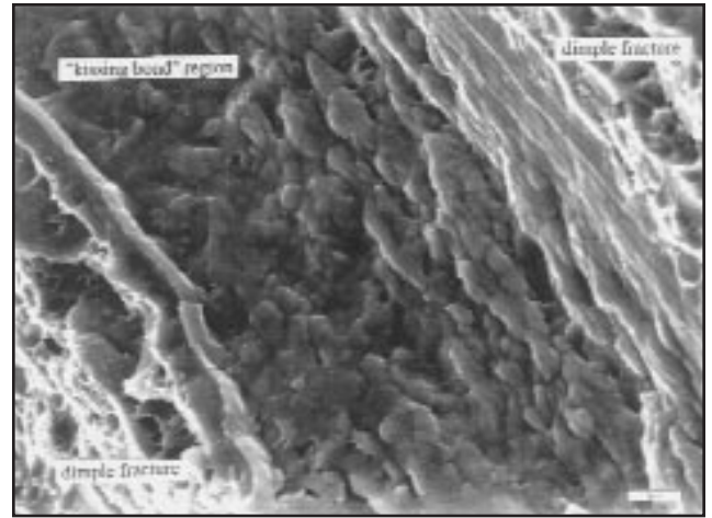
Fig. 14 — Close-up of the center kissing bond region of the specimen in Fig. 13.
