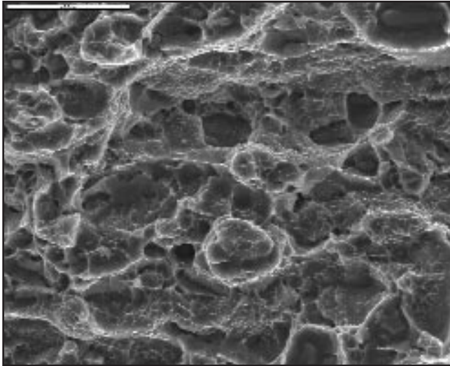
Fig. 7 — Dimples in a AA6082 base material specimen
