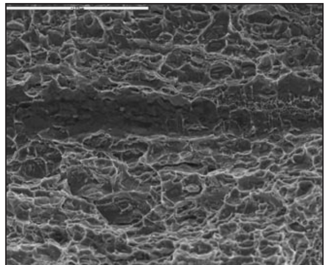
Fig. 10 — Overview of the fracture surface of a longitudinal weld in AA6082 with kissing bond showing in the center.
