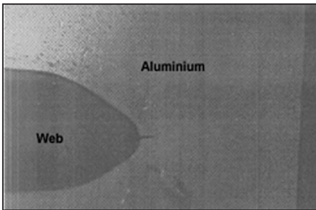
Fig. 5 — Split metal in the welding chamber, right behind the web; extrusion direction is from the left to the right. The dark gray body to the left is the web.
