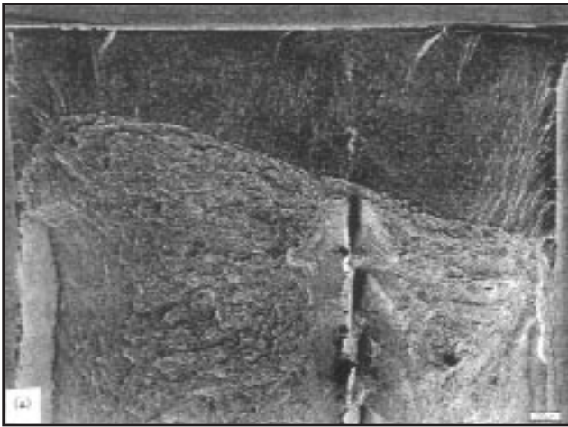
Fig. 13 — Fracture surface of a friction stir weld in AA6082 showing vertically lined-up, tear-shaped kissing bonds.
