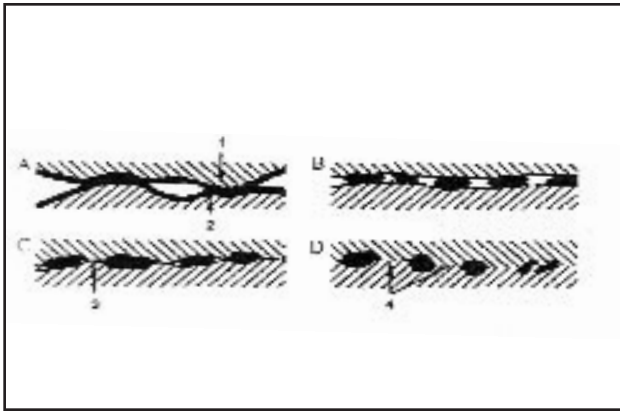
Fig. 3 — Four stages of transverse welding by Akeret.
