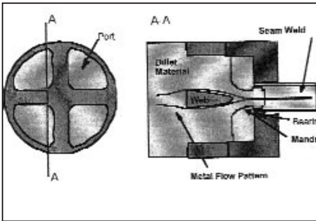
Fig. 1 — Schematic representation of longitudinal weld formation.
