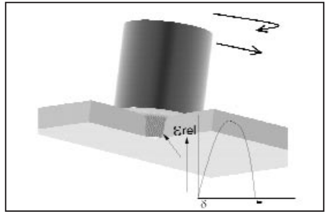
Fig. 4 — Shear zone around the pin in FSW.
