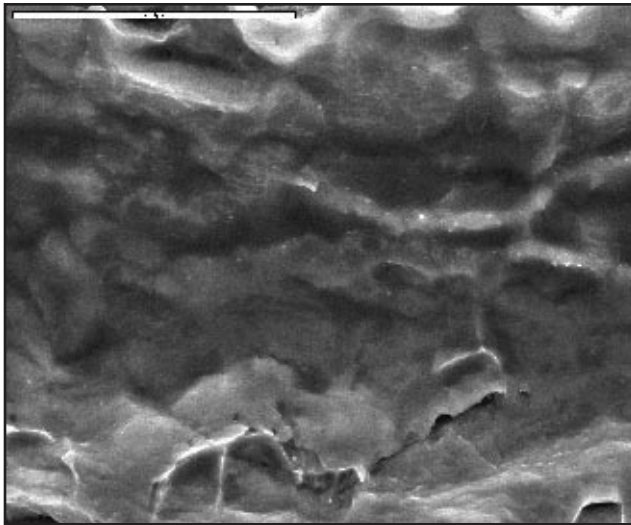
Fig. 11 — Close-up of the kissing bond in a longitudinal weld specimen in AA6082.
