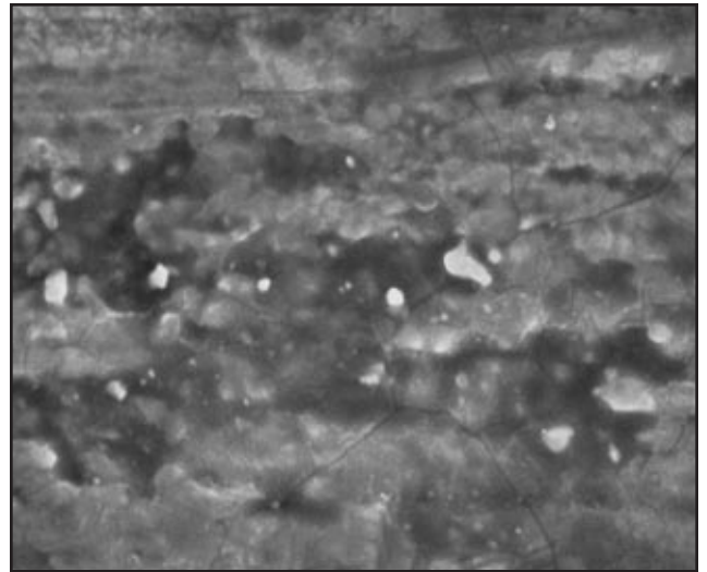
Fig. 12 — Extruded surface of a base material specimen of AA6082.
