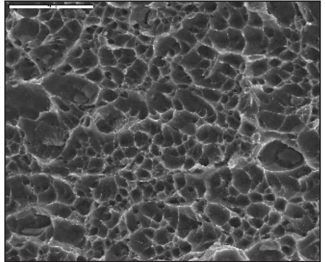
Fig. 8 — Dimples in a transverse weld specimen in AA6082
