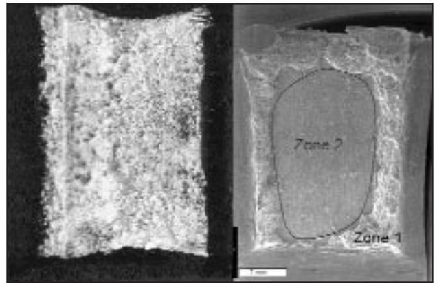
Fig. 6 — A — The fracture surface of a tensile tested transverse weld specimen in AA6060 aluminum alloy (by stereo microscope). B — The fracture surface (by SEM) of a Charpy-tested specimen of the same transverse weld at the same position along the extruded length
