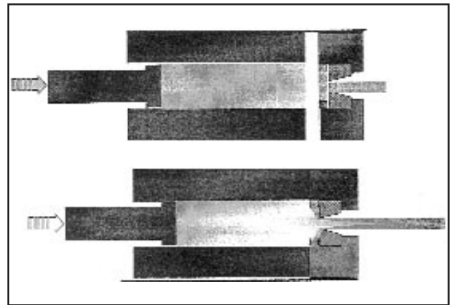
Fig. 2 — Schematic representation of transverse weld formation.
