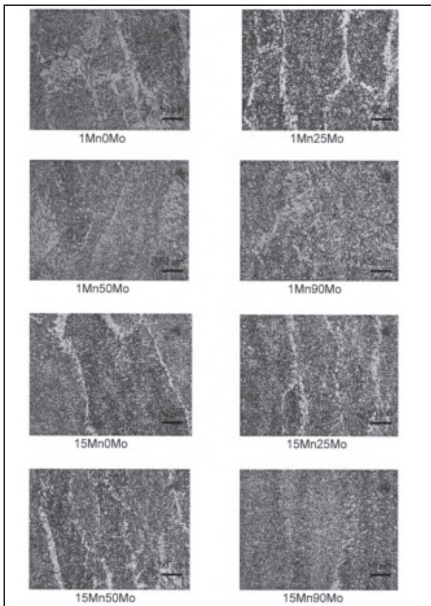
Fig. 5 — As-welded condition columnar zone microphotographs.
