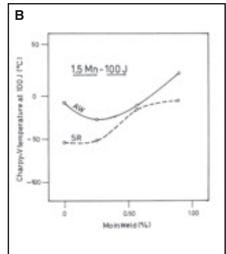
Fig. 13 — Test temperature for 100 J absorbed energy. A — 1% Mn; B — 1.5% Mn.
