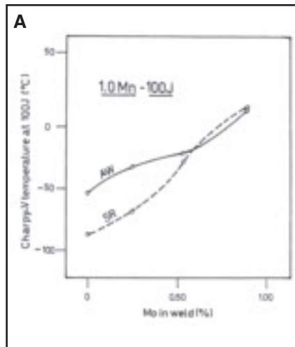
Fig. 13 — Test temperature for 100 J absorbed energy. A — 1% Mn; B — 1.5% Mn.
