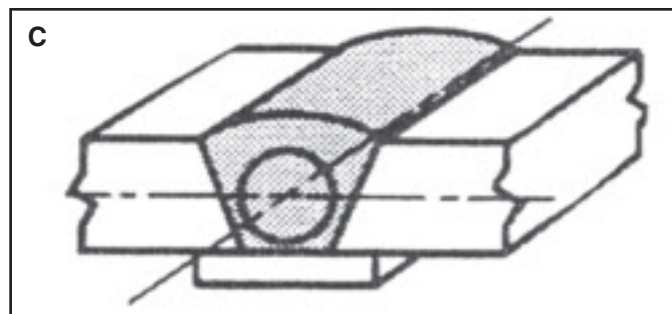
Fig. 1 — A — Test plate showing coupon design and locations of test specimens; B — location of impact test specimen and Charpy V-notch test location; C — location of all-weld-metal tension test specimen.
