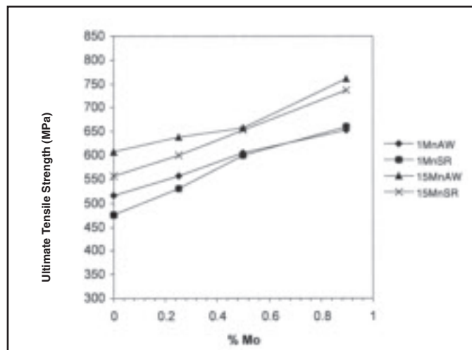
Fig. 10 — Effect of molybdenum on ultimate tensile strength.
