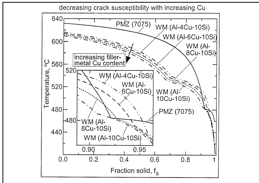
Fig. 8 — T-f_s curves predicting reduction of liquation-cracking susceptibility of 7075 welds by increasing Cu content in filler metal Al-xCu-10Si to minimize extent of WM f_s > PMZ f_s during solidification, 65% dilution. Curves calculated using Pandat software of CompuTherm LLC (Ref. 28).
