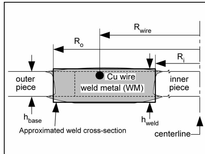
Fig. 2 — Approximated weld transverse cross section.
