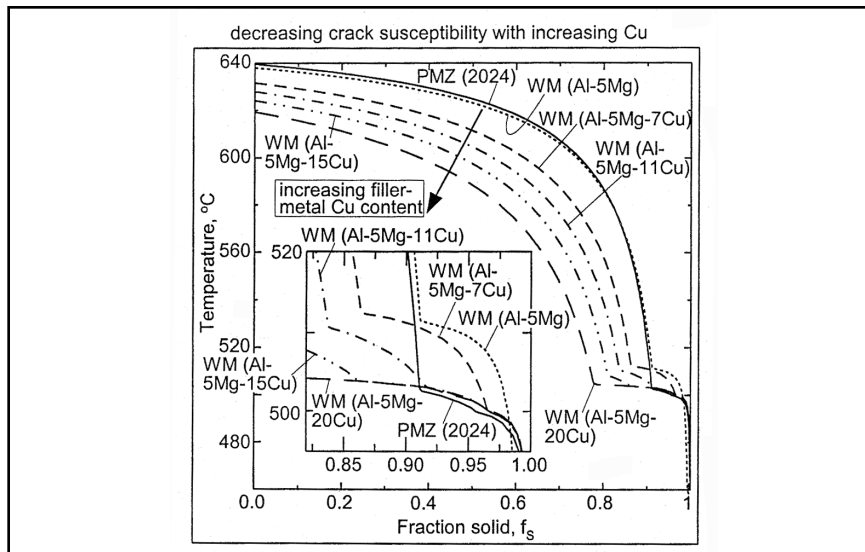
Fig. 13 — T-f_s curves predicting reduction of liquation-cracking susceptibility of 2024 welds by increasing Cu content in filler metal Al-5Mg-xCu to minimize the extent of WM f_s > PMZ f_s during solidification, 65% dilution. Curves calculated using Pandat software of CompuTherm LLC (Ref. 28).
