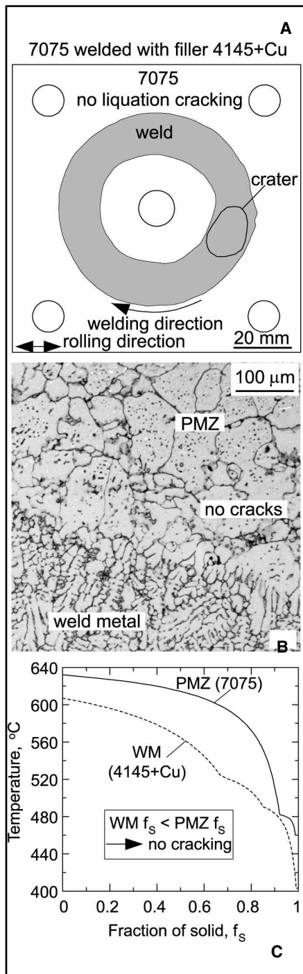
Fig. 9 — Alloy 7075 welded with filler metal 4145 plus extra Cu. A — Overview; B — micrograph; C — T-f_s curves. Elimination of cracking confirms effect of increasing filler-metal Cu content on reducing crack susceptibility predicted by T-f_s curves. Curves calculated using Pandat software of CompuTherm LLC (Ref. 28).
