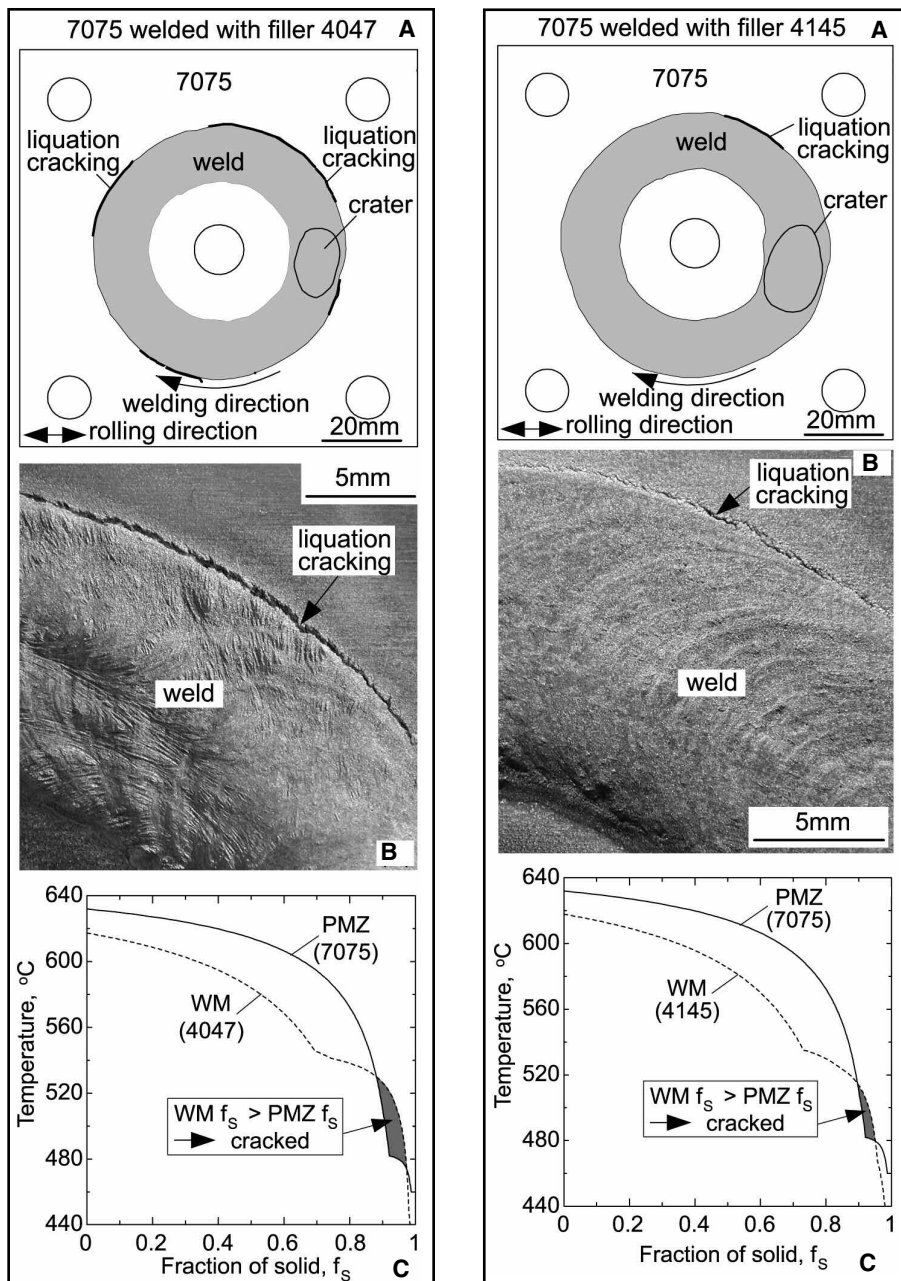
Fig. 6 — Liquation cracking in Alloy 7075 welded with filler metal 4047. A — Overview; B — macrograph; C — T-f s curves. Crack susceptibility predicted by T-f s curves confirmed. Curves calculated using Pandat of CompuTherm LLC (Ref. 28).
