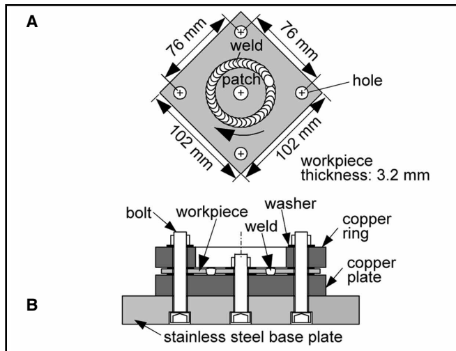
Fig. 1 — Circular-patch welding. A — Top view of workpiece; B — side view of apparatus.
