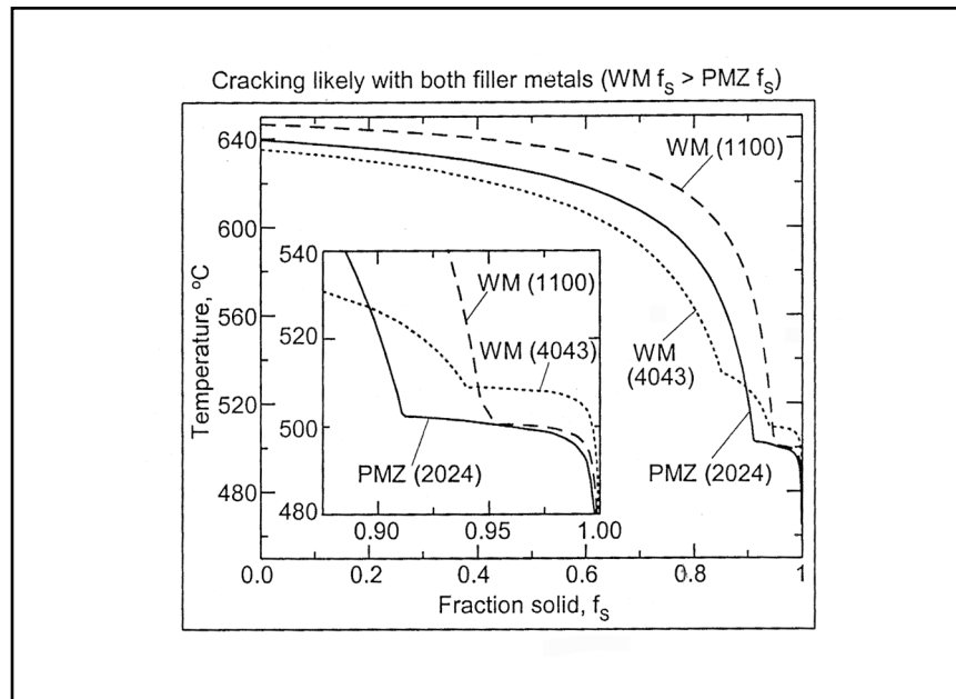
Fig. 10 — T-f_s curves predicting crack susceptibility of 2024 welds made with filler metals 1100 and 4043 at 65% dilution of filler metal by base metal. Curves calculated using Pandat software of CompuTherm LLC (Ref. 28).
