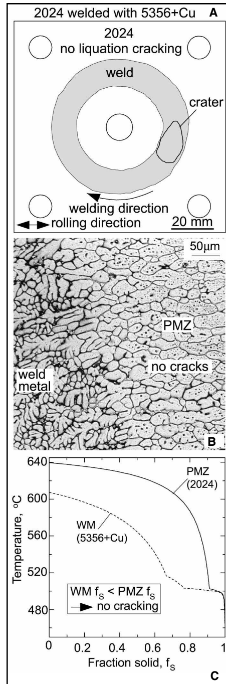
Fig. 14 — Alloy 2024 welded with filler metal 5356 plus extra Cu. A — Overview; B — transverse micrograph; C — T-f_s curves. Elimination of cracking confirms effect of increasing filler-metal Cu content on reducing crack susceptibility predicted by T-f_s curves. Curves calculated using Pandat software of CompuTherm LLC (Ref. 28).
