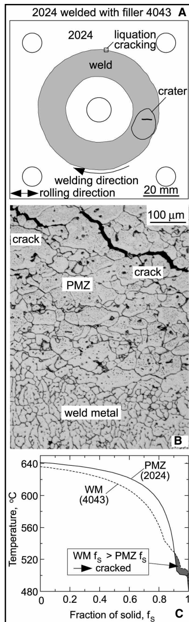
Fig. 12 — Liquation cracking in Alloy 2024 welded with filler metal 4043. A — Overview; B — micrograph; C — T-f_s curves. Crack susceptibility predicted by T-f_s curves confirmed. Curves calculated using Pandat software of CompuTherm LLC (Ref. 28).
