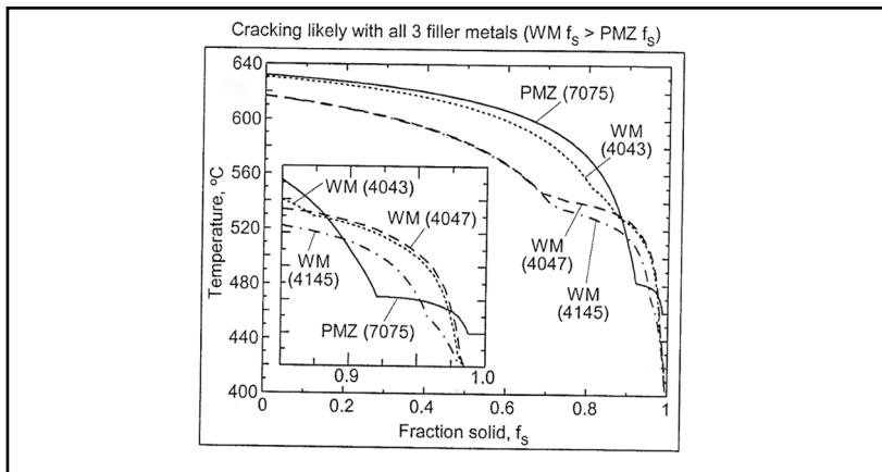
Fig. 4 — T-f_s curves predicting crack susceptibility of 7075 welds made with filler metals 4043, 4047, and 4145 at 65% dilution of filler metal by base metal. Curves calculated using Pandat software of CompuTherm LLC (Ref. 28).
