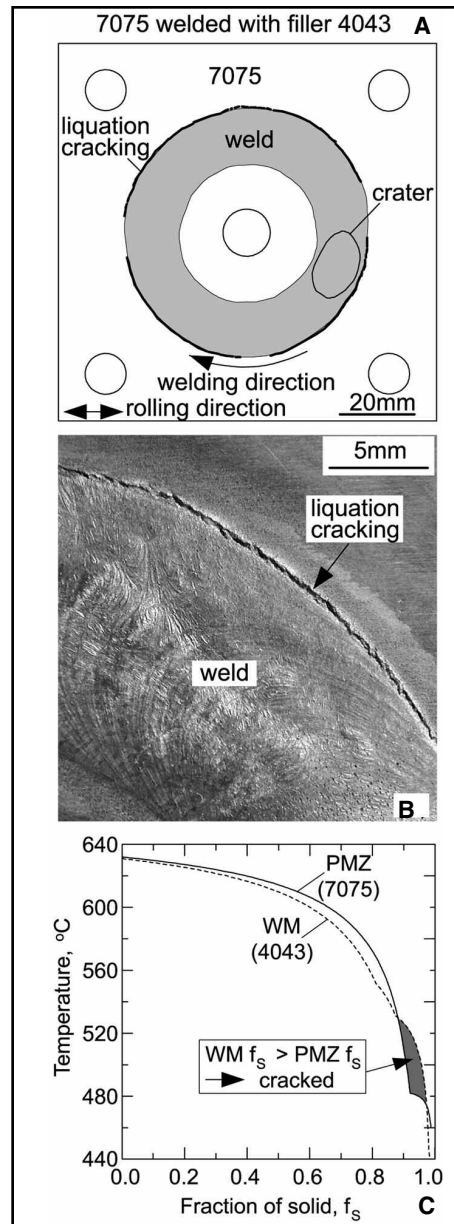
Fig. 5 — Liquefaction cracking in Alloy 7075 welded with filler metal 4043. A — Overview; B — macrograph; C — T-f_s curves. Crack susceptibility predicted by T-f_s curves confirmed. Curves calculated using Pandat software of CompuTherm LLC (Ref. 28).
