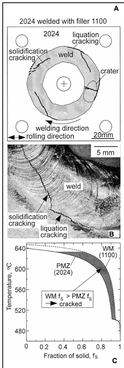
Fig. 11 — Liquation cracking in Alloy 2024 welded with filler metal 1100. A — Overview; B — macrograph; C — T-f_s curves. Crack susceptibility predicted by T-f_s curves confirmed. Curves calculated using Pandat of CompuTherm LLC (Ref. 28).
