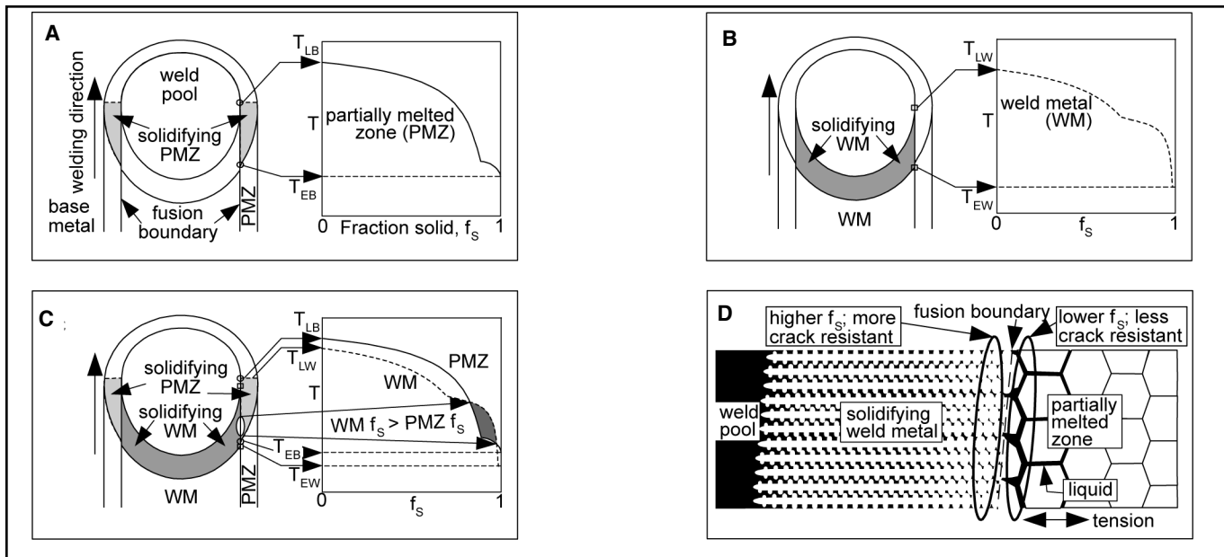
Fig. 3 — T - f_s curves along fusion boundary. A — Solidifying PMZ; B — solidifying WM; C — superimposed to show region of WM f_s > PMZ f_s ; D — example microstructure of WM f_s > PMZ f_s .
