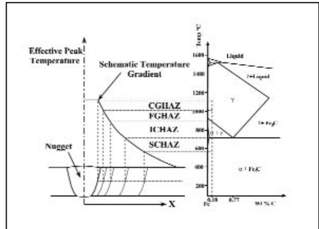
Fig. 9 — Schematic illustration of the different regions of the HAZ of a friction stir weld on mild steel and their relation to effective temperatures in the Fe-Fe 3 C binary system.
