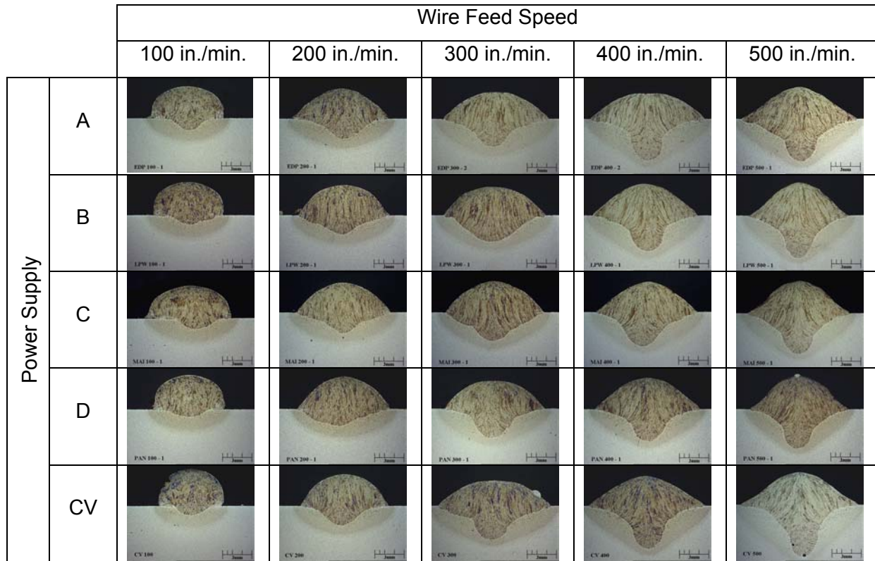
Figure 3. Macro Section Map for Simulated GMAW-P Waveforms
