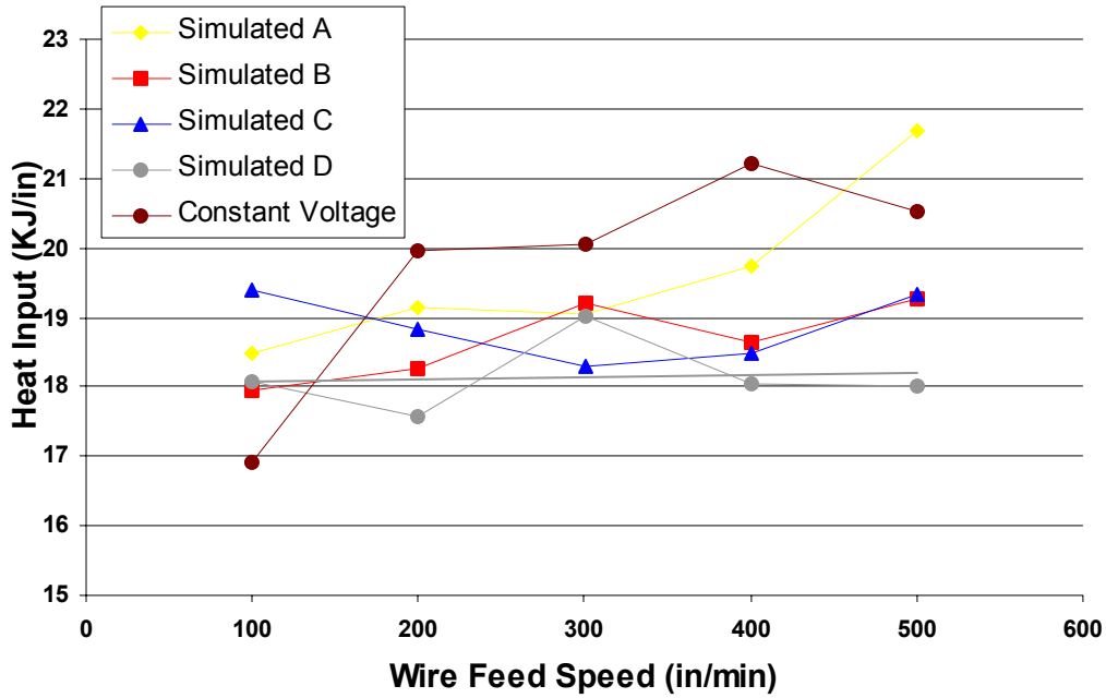
Figure 2. Heat Input (based on AIP) versus Wire Feed Speed for Simulated GMAW-P Waveforms.
