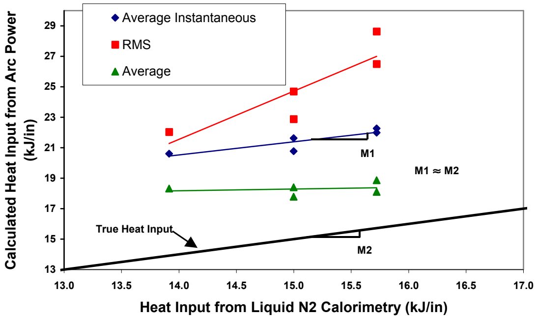
Figure 1. Graph Comparing Calculated Heat Input to Actual Heat Input for GMAW-P
